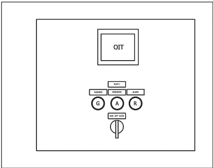
3 TANK NO.4 PUMPHOUSE - RTU DEVICE ELEVATION NOT TO SCALE
