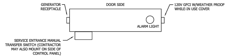
3 WEST SIDE LIFT STATION - CABINETS PLAN VIEW NOT TO SCALE
