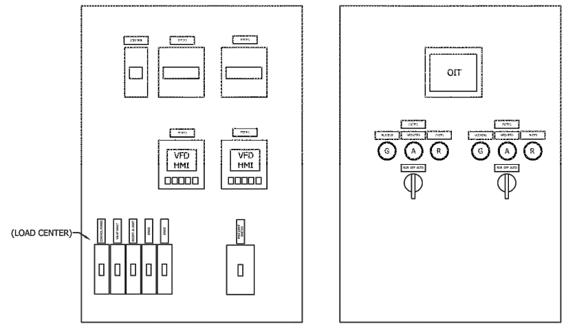
2 WEST SIDE LIFT STATION - CONTROL CABINET INNER DOOR - PROPOSED LAYOUT NOT TO SCALE
