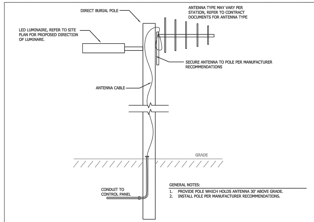
5 WEST SIDE LIFT STATION - ANTENNA POLE DETAIL NOT TO SCALE
