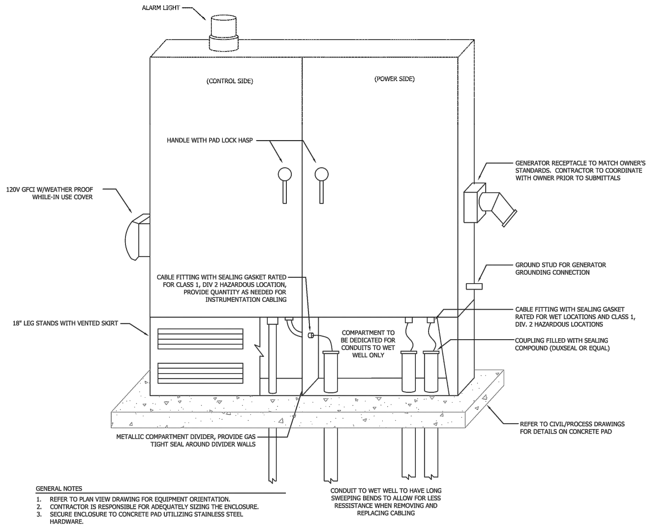
1 WEST SIDE LIFT STATION - CONTROL PANEL ELEVATION NOT TO SCALE
