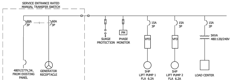
4 WEST SIDE LIFT STATION - ONE-LINE DIAGRAM NOT TO SCALE
