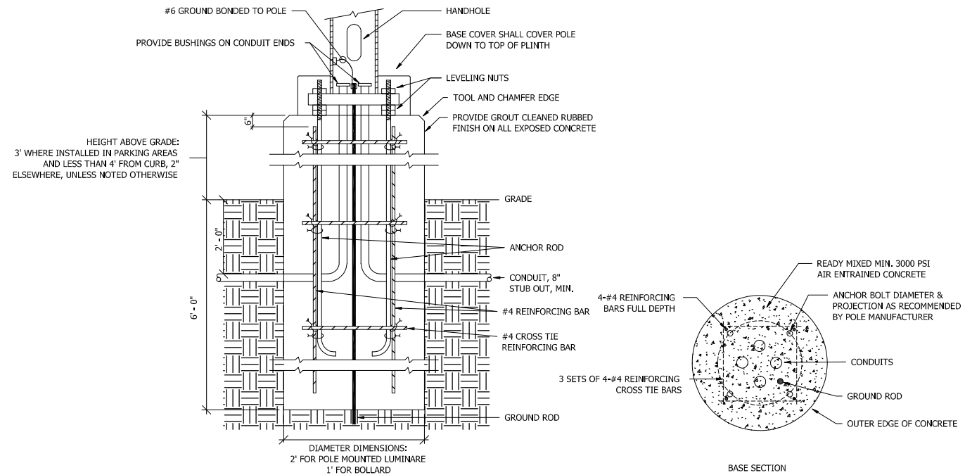
2 LIGHT POLE BASE DETAIL NOT TO SCALE
