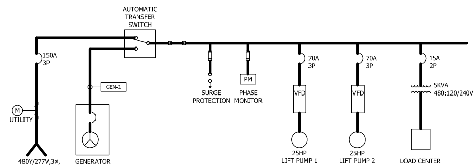
5 ONE-LINE DIAGRAM NOT TO SCALE
