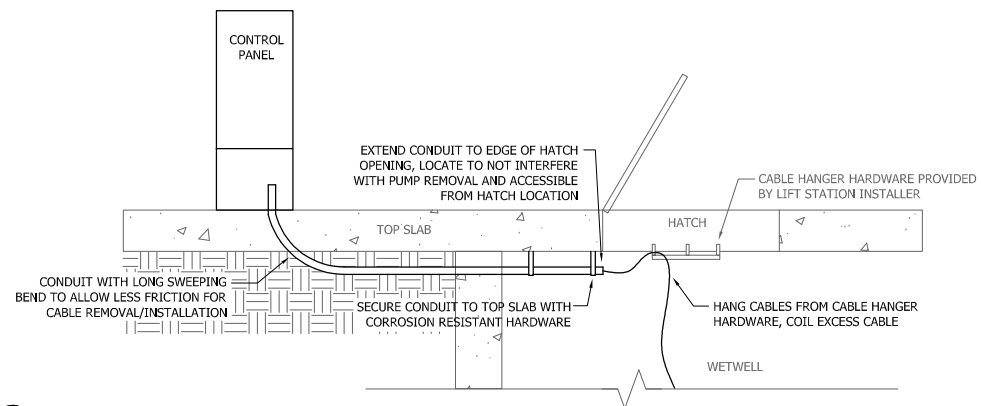
6 WETWELL CONDUIT INSTALLATION DETAIL (TYPICAL) NOT TO SCALE
