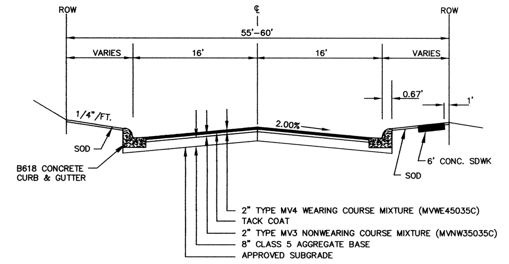
TYPICAL STREET SECTION ZANE AVENUE
