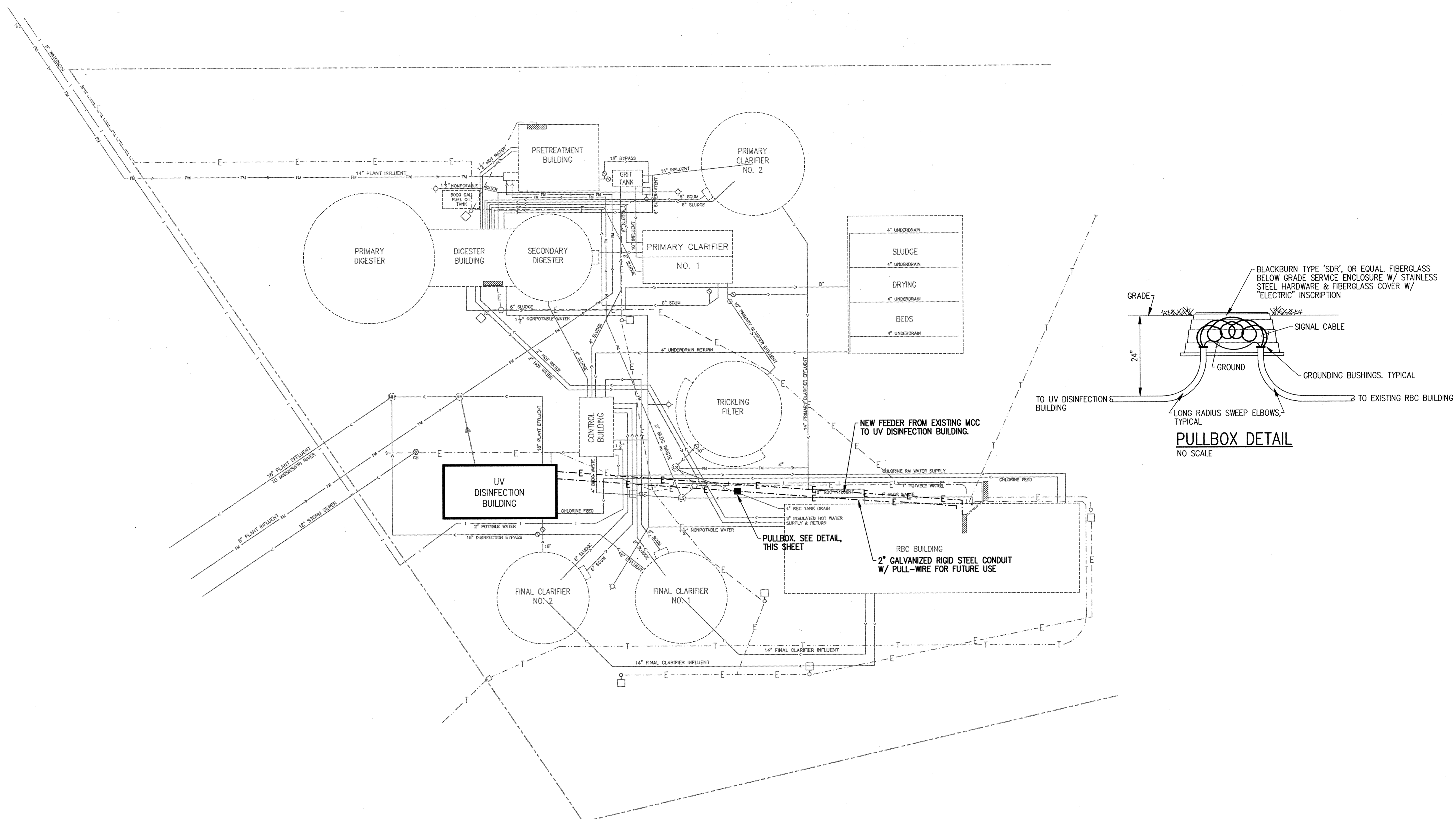
North ELECTRICAL SITE PLAN SCALE: 1"=20' 0 10 20 40 60 Graphic Scale
