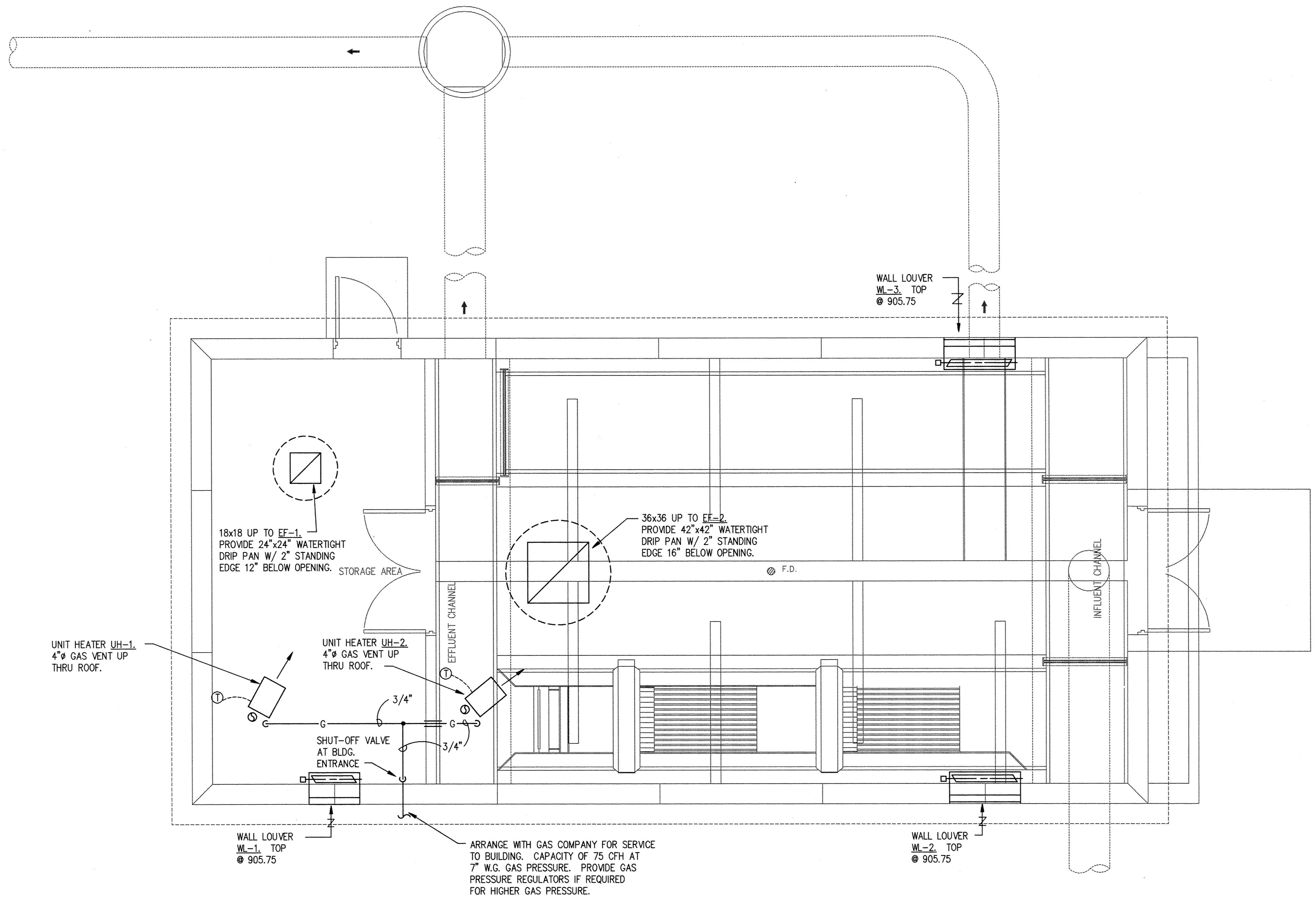
DISINFECTION BUILDING MECHANICAL PLAN SCALE: 3/8"=1'-0"
