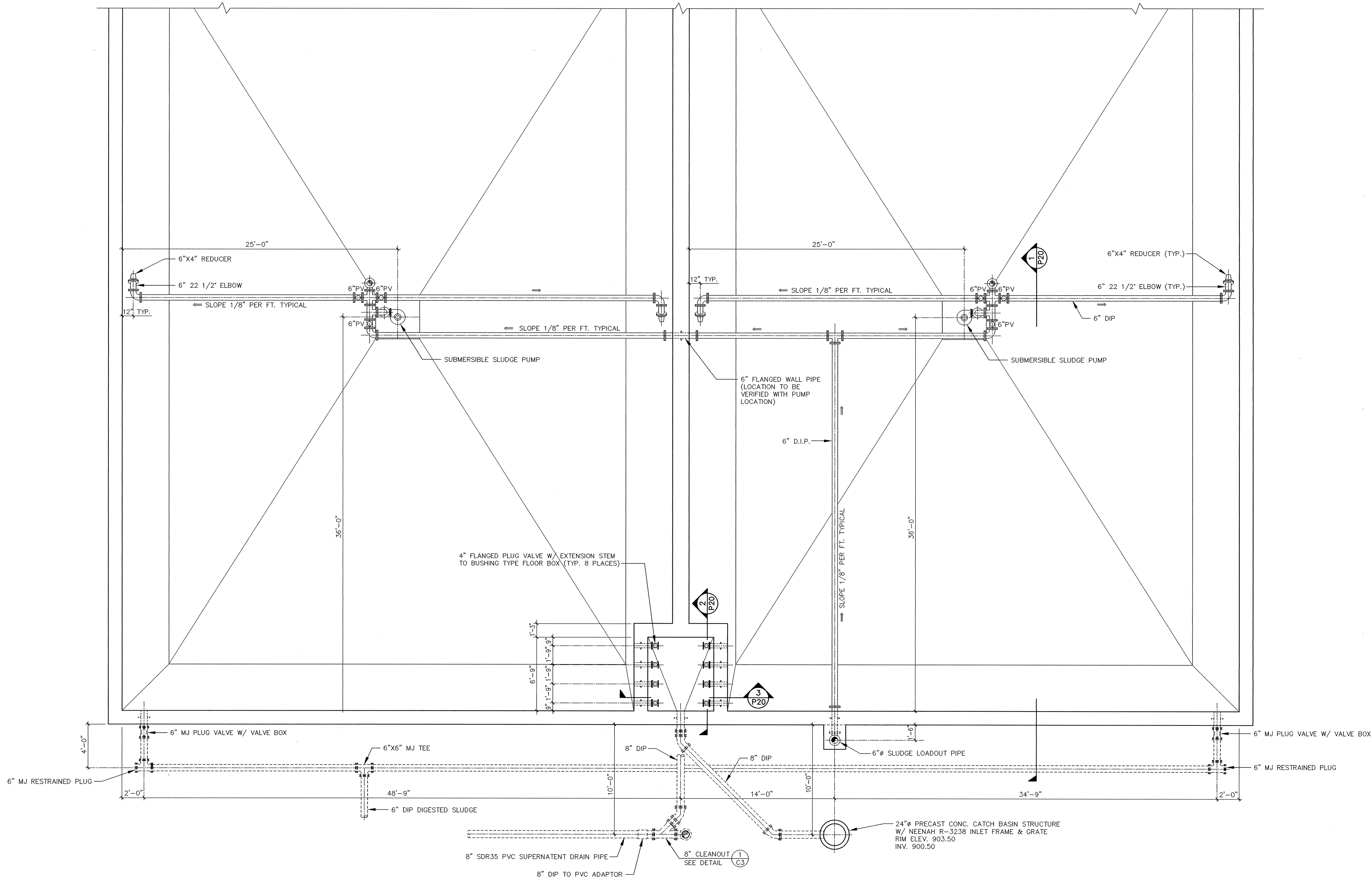
DIGESTED SLUDGE STORAGE TANK PLAN @ BOTTOM OF D.T. Scale: 1/4" = 1'-0"
