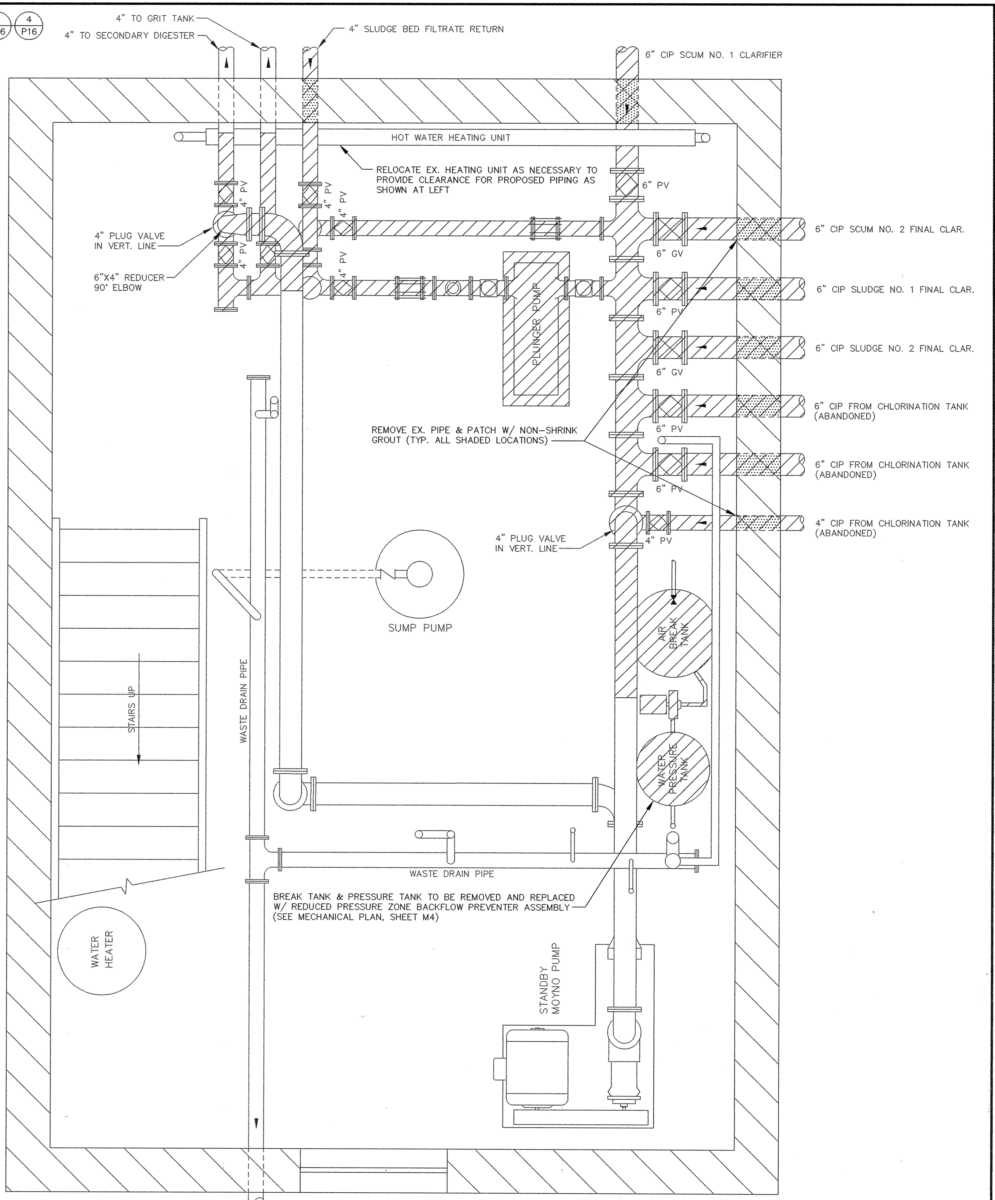
CONTROL BLDG. EX. BASEMENT PIPING PLAN Scale 3/4" = 1'-0"
