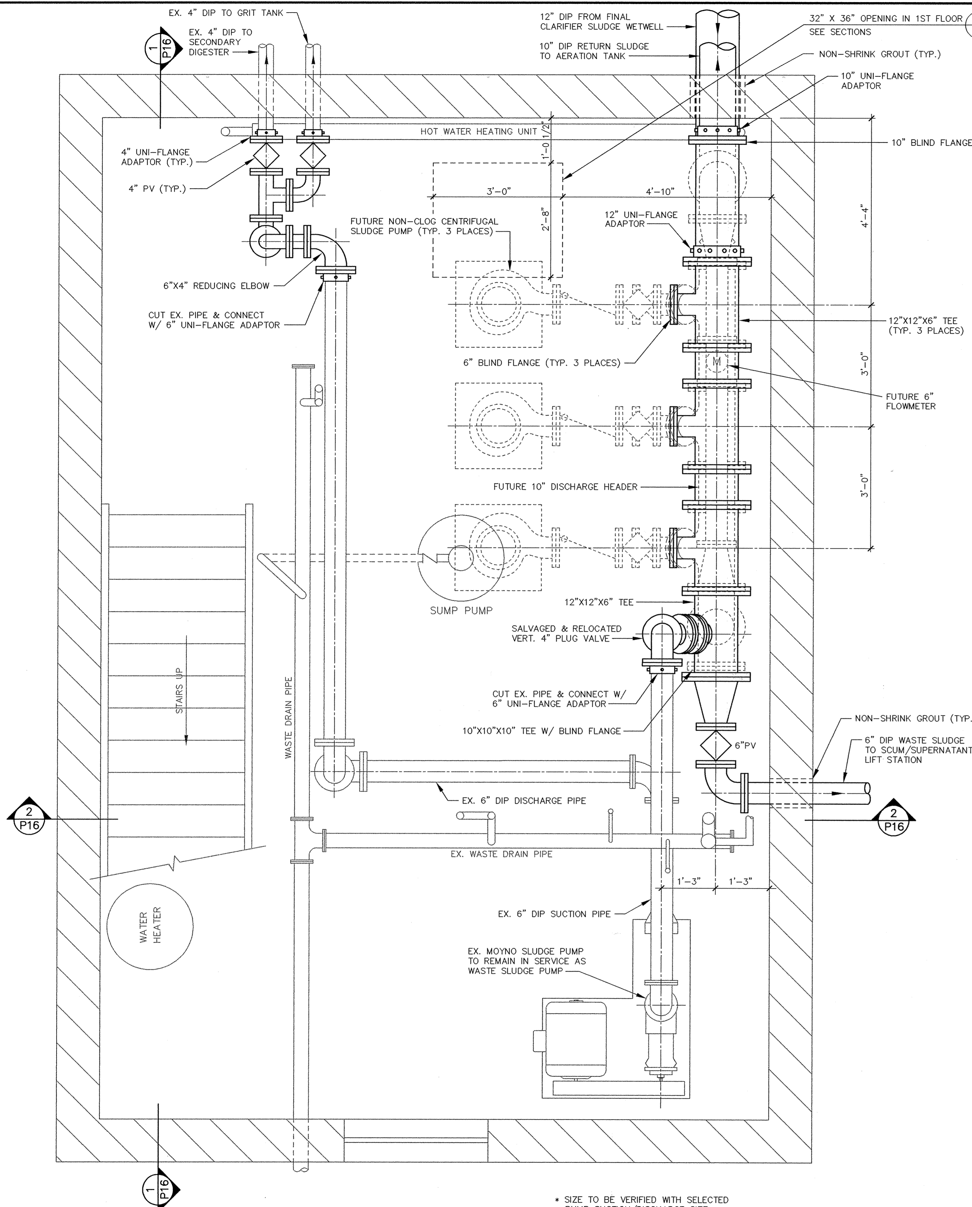
CONTROL BLDG. PROPOSED BASEMENT PIPING PLAN Scale 3/4" = 1'-0"
