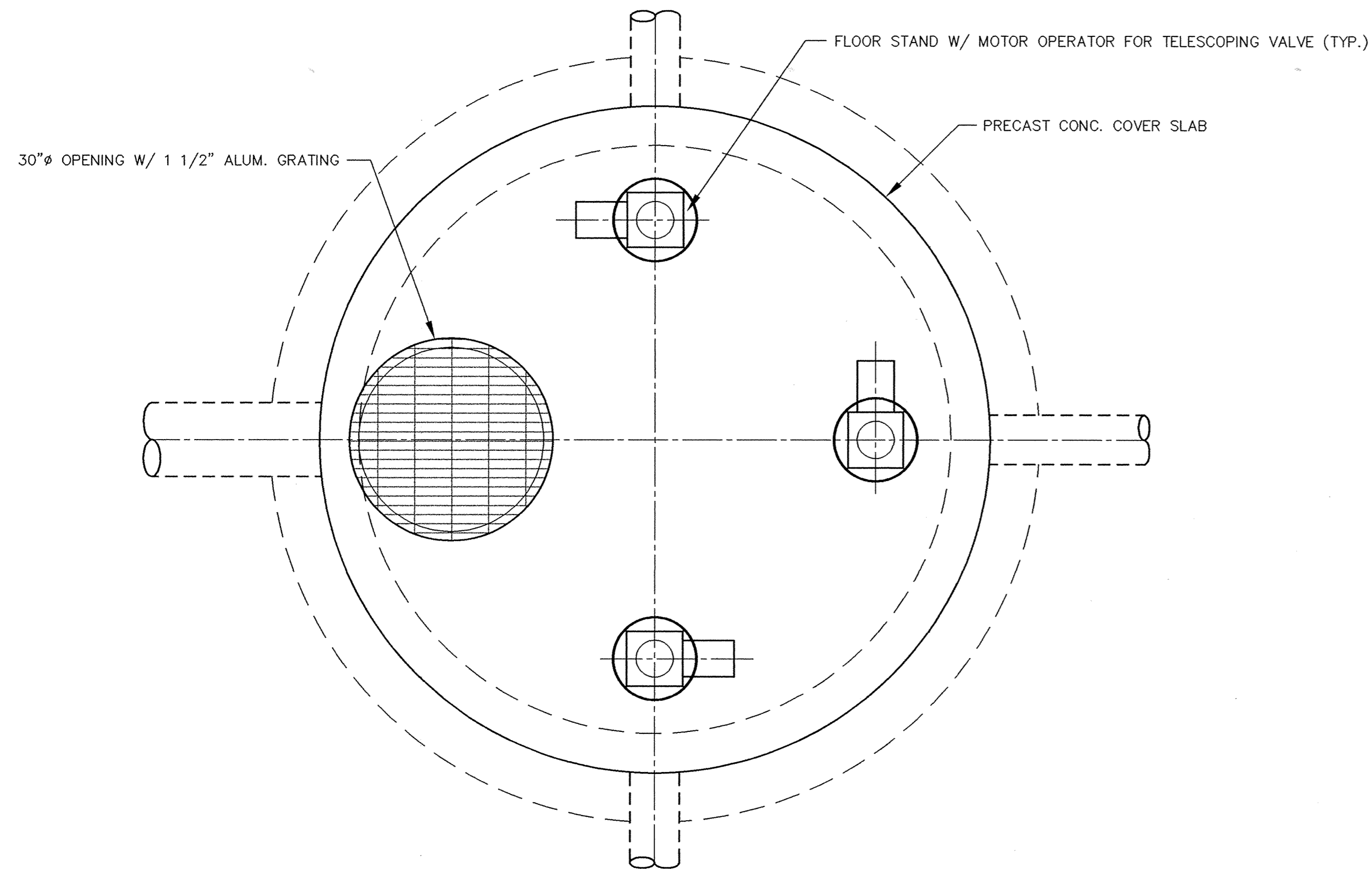
FINAL CLARIFIER SLUDGE WETWELL PLAN Scale: 3/4" = 1'-0"
