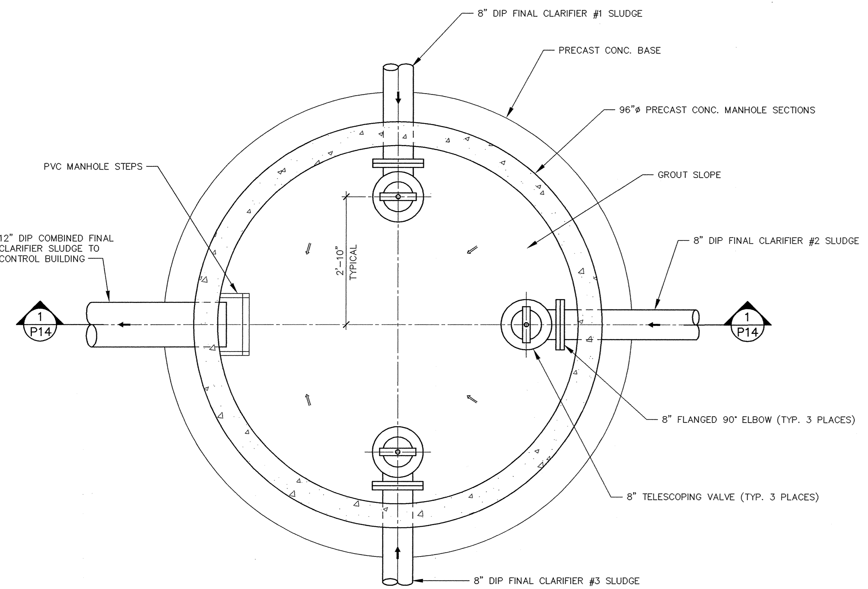
FINAL CLARIFIER SLUDGE WETWELL SECTIONAL PLAN Scale: 3/4" = 1'-0"
