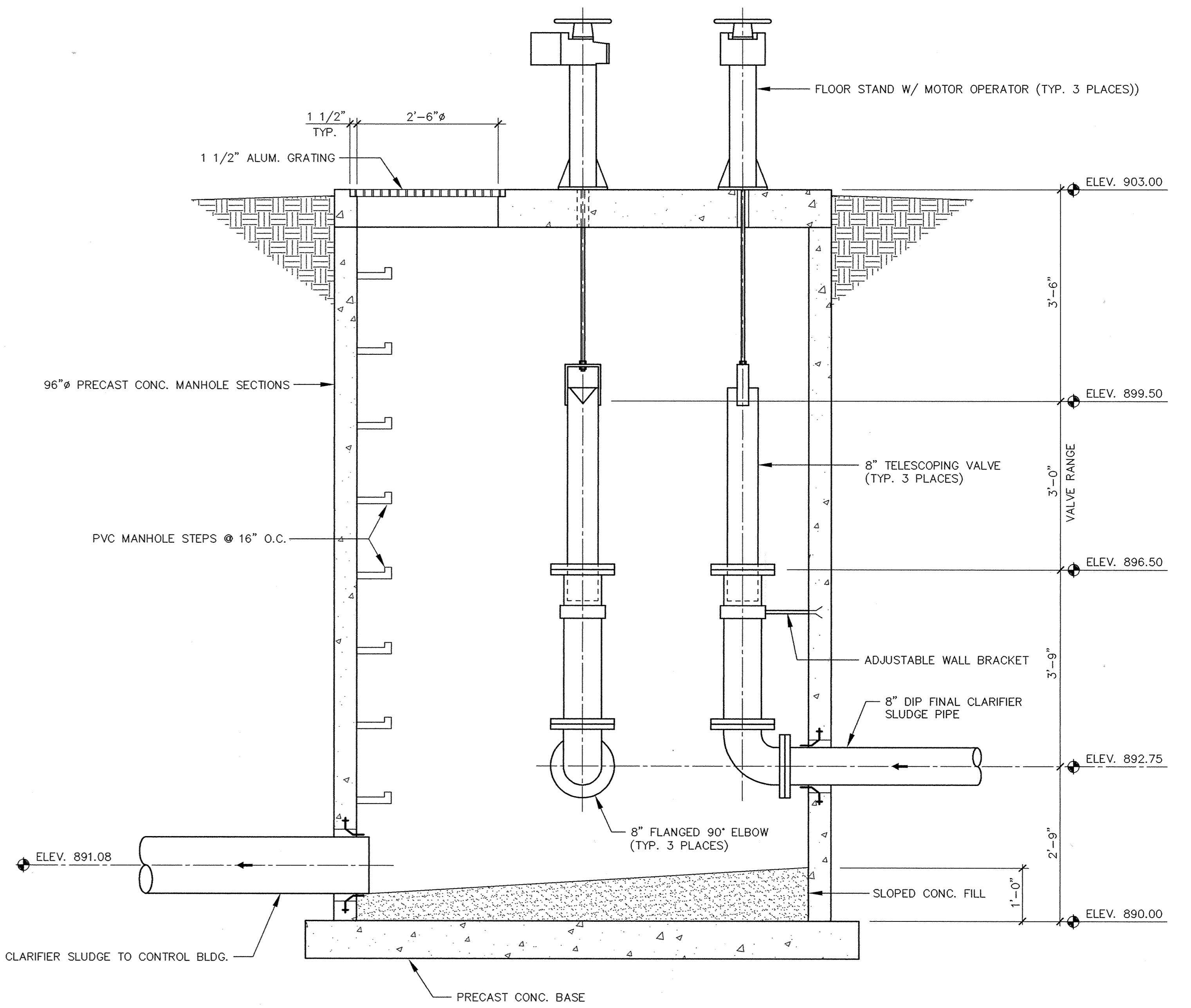
FINAL CLARIFIER SLUDGE WETWELL SECTION Scale: 3/4" = 1'-0"
