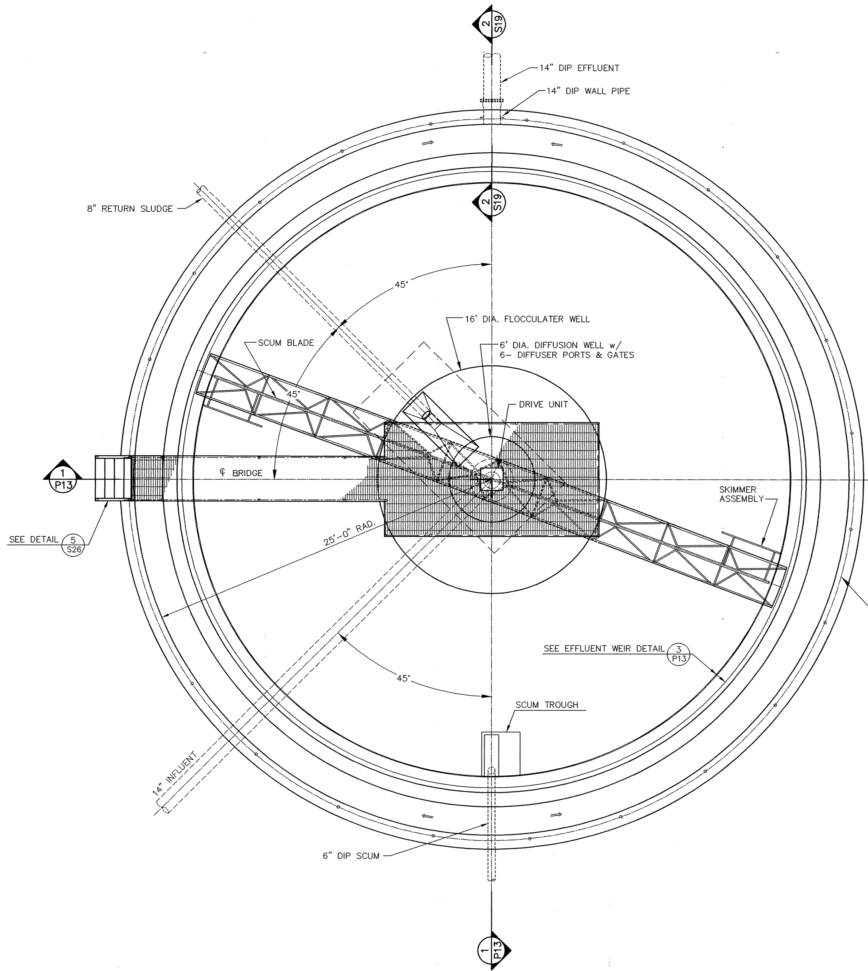
FINAL CLARIFIER PLAN @ GRADE Scale: 1/4" = 1'-0"
