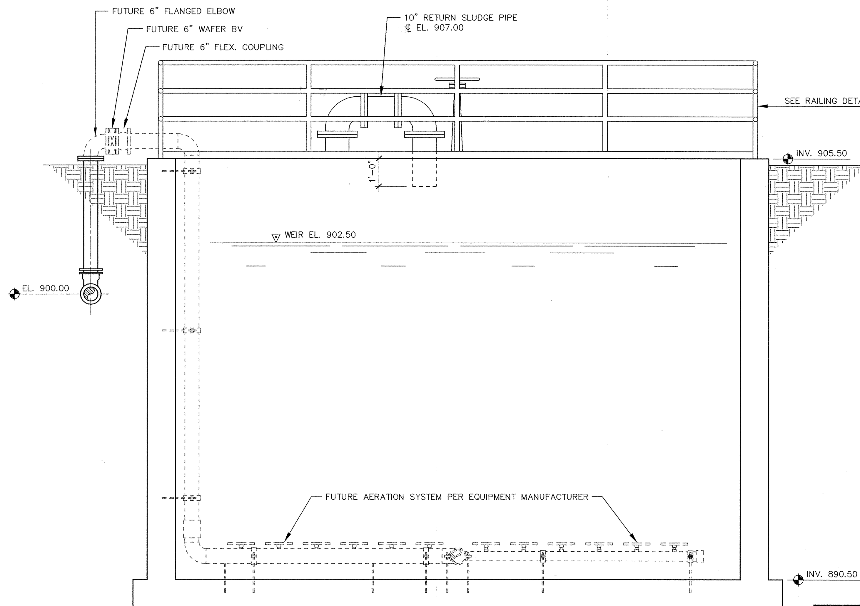
AERATION TANK SECTION 2 Scale: 1/2" = 1'-0"
