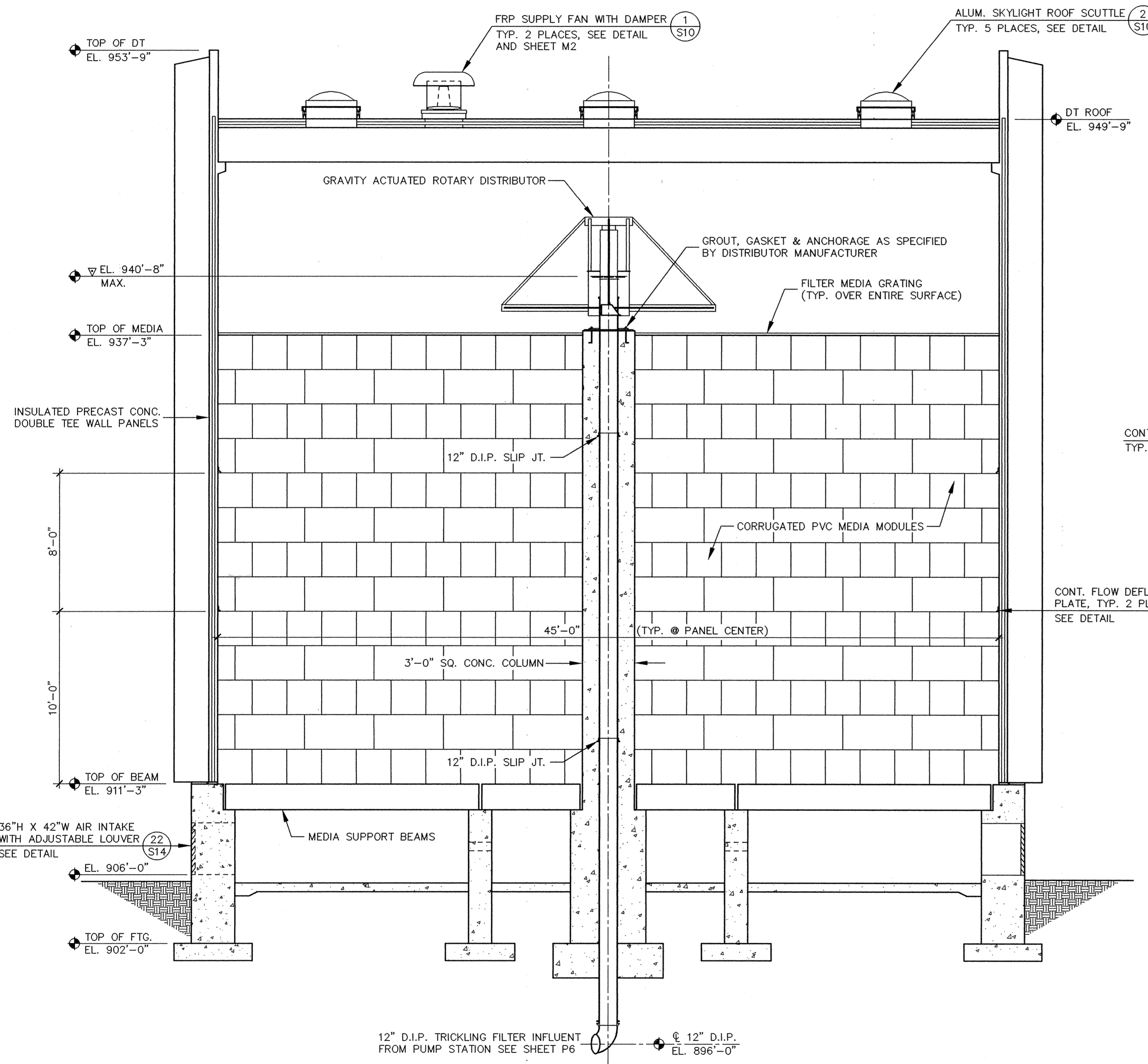
TRICKLING FILTER SECTION 1 Scale: 1/4" = 1'-0" P7
