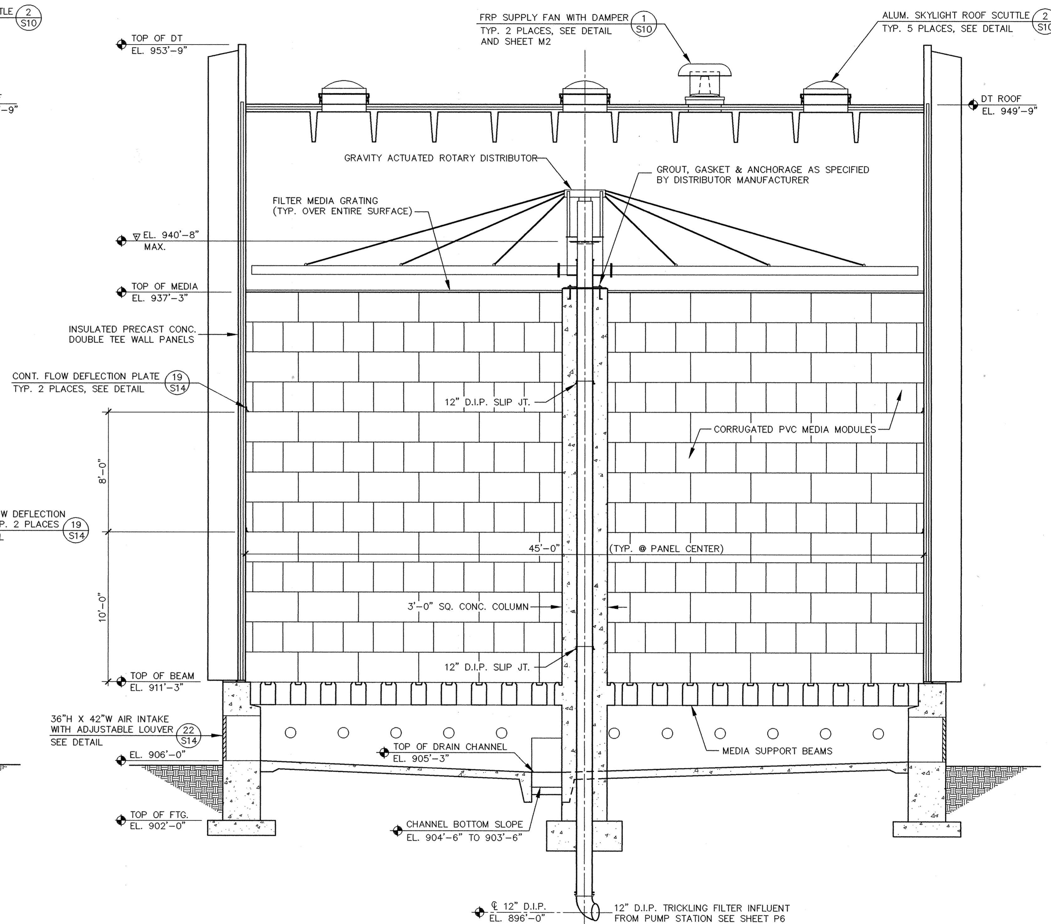
TRICKLING FILTER SECTION 2 Scale: 1/4" = 1'-0" P7
