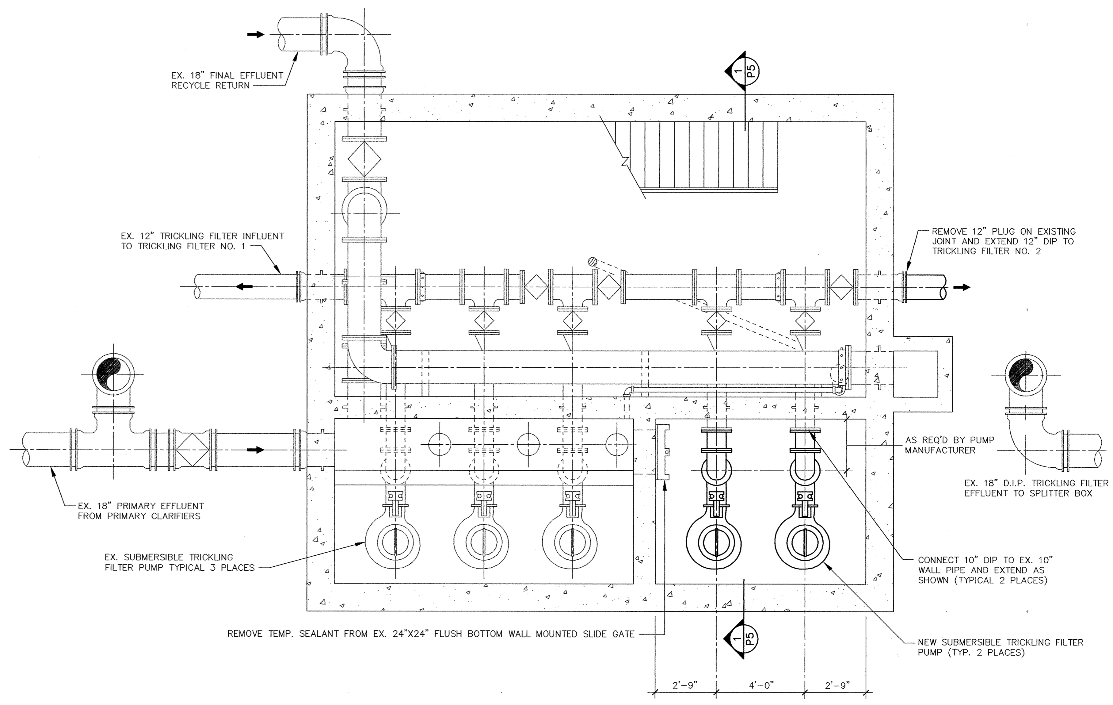
TRICKLING FILTER PUMP STATION PLAN @ EL. 900.00 Scale: 3/8" = 1'-0"
