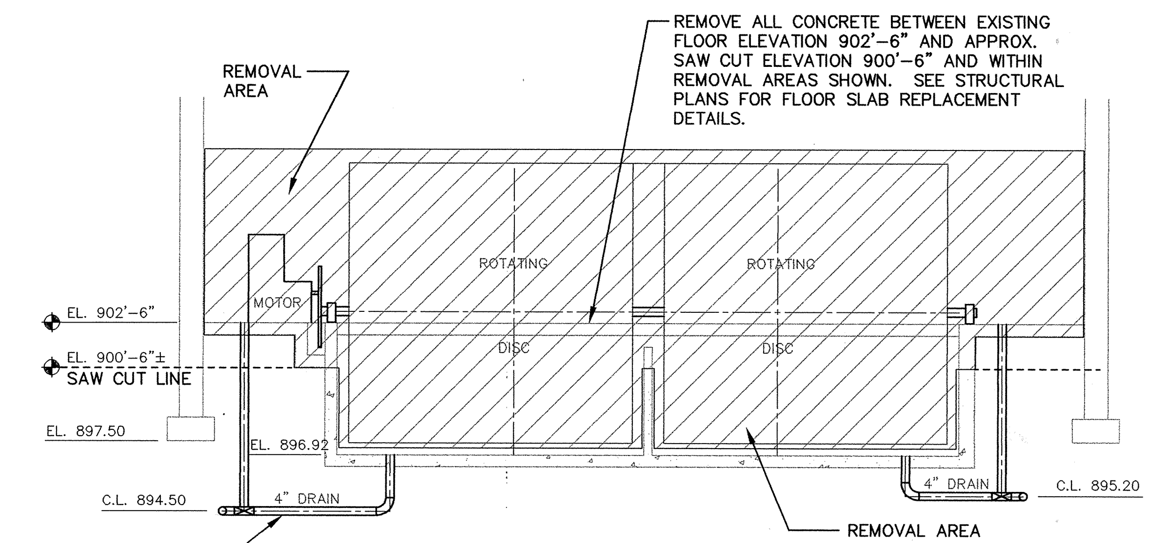
MAIN BUILDING DEMOLITION - SECTION 2 Scale: 1/4" = 1'-0"
