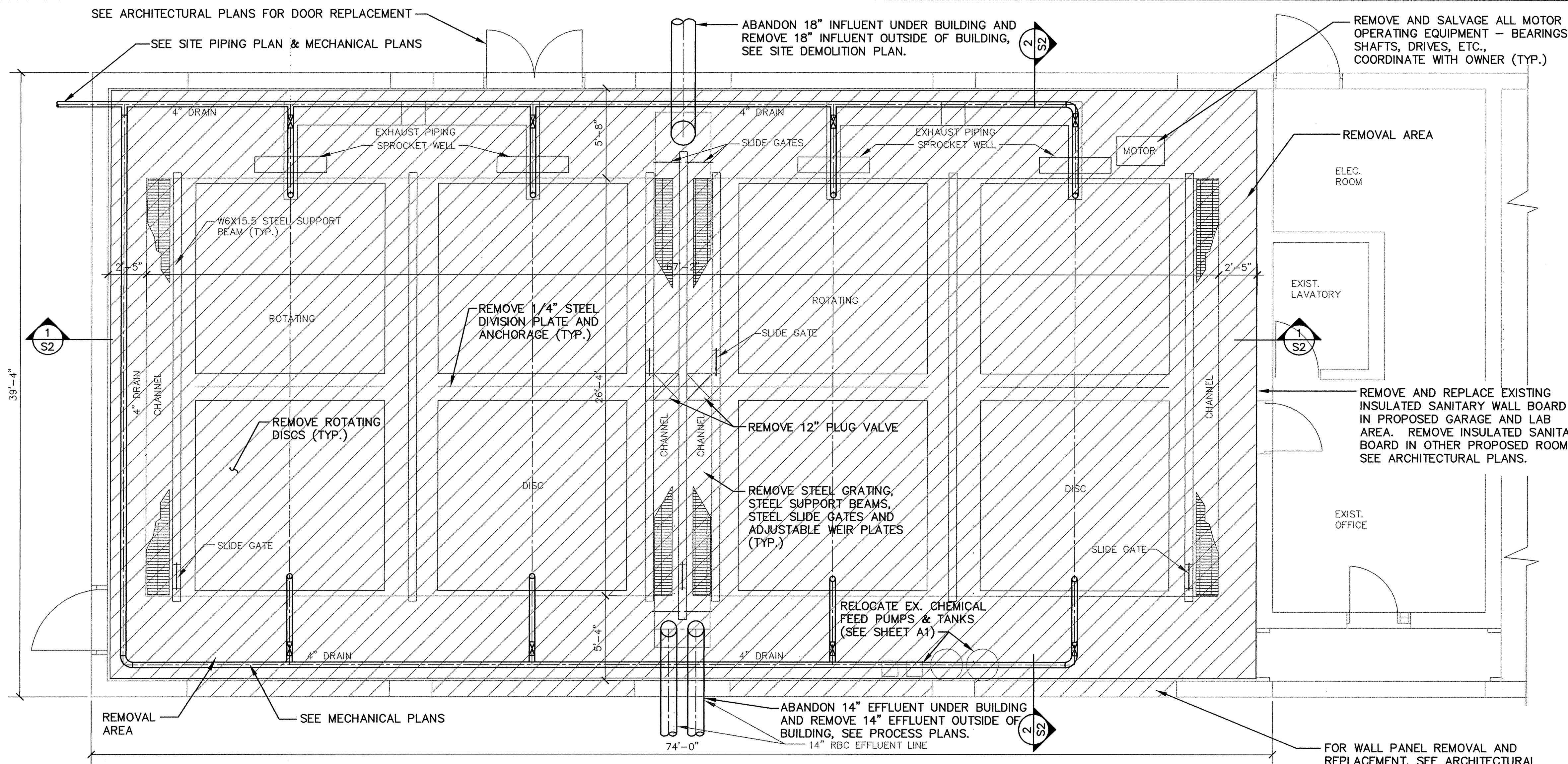
MAIN BUILDING DEMOLITION - PLAN Scale: 1/4" = 1'-0"
