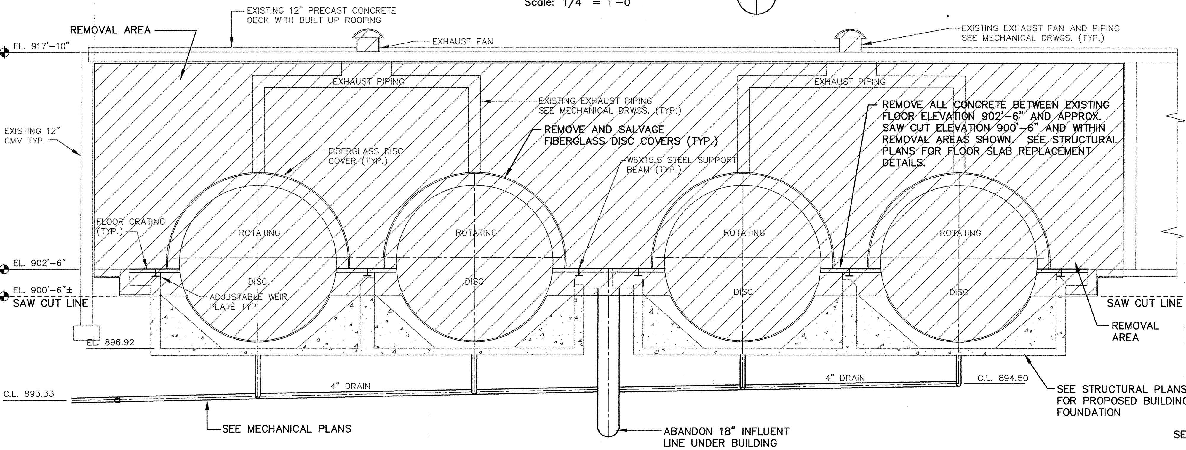
MAIN BUILDING DEMOLITION - SECTION 1 Scale: 1/4" = 1'-0"
