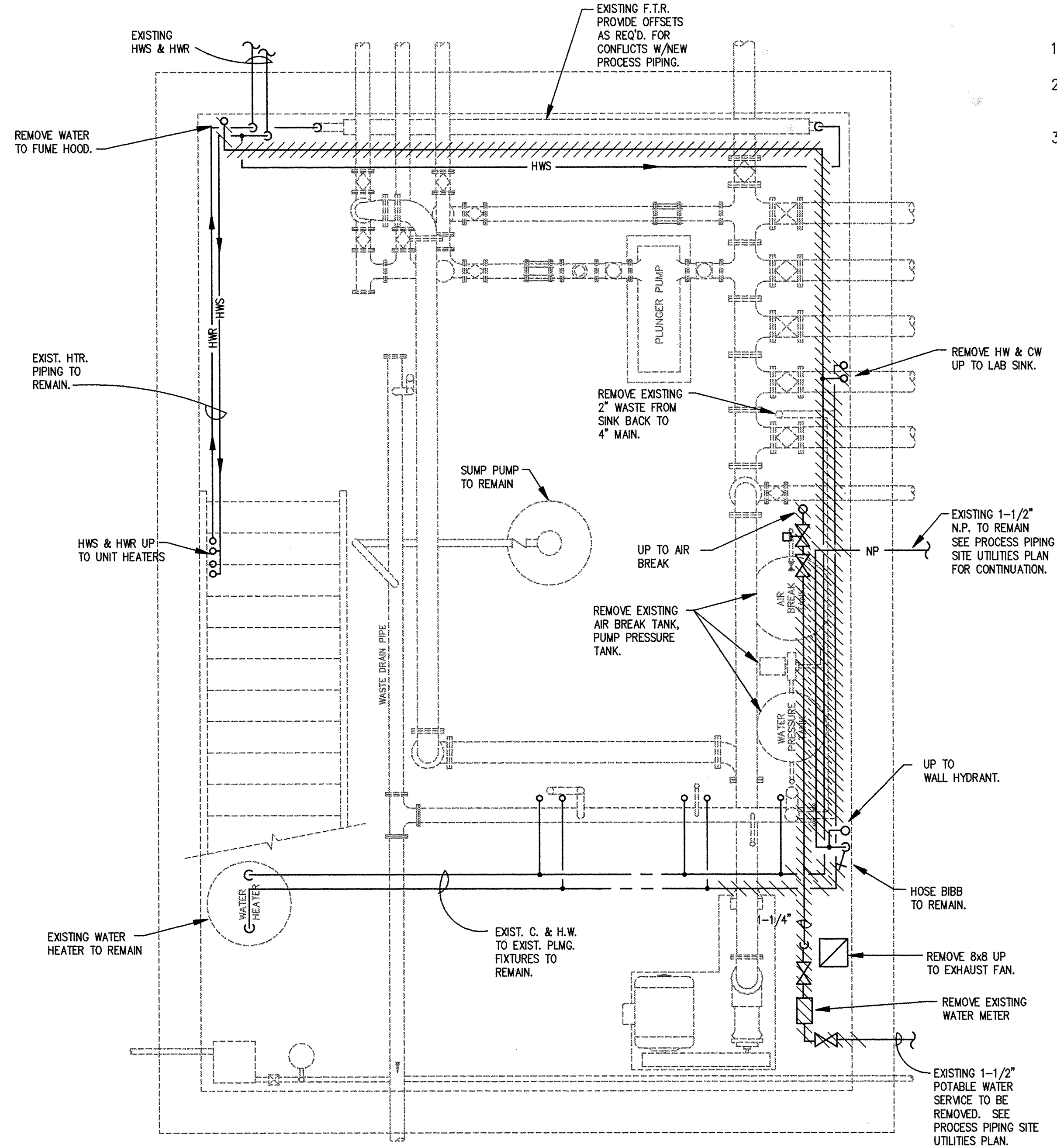
North ↑ 2 CONTROL BUILDING MECHANICAL DEMOLITION PLAN M4 SCALE: 1/2"=1'-0" BASEMENT FLOOR
