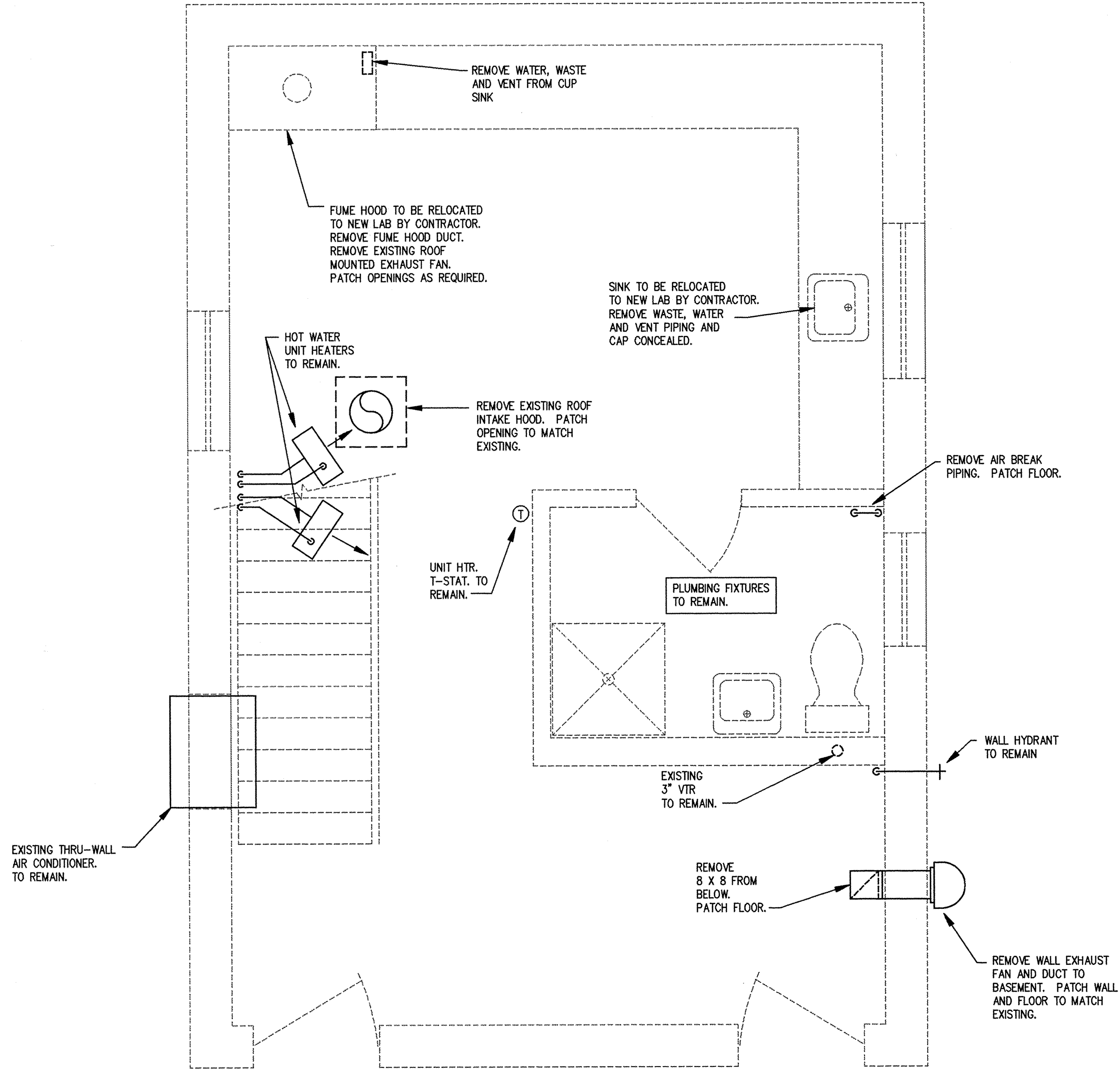
North ↑ 1 CONTROL BUILDING MECHANICAL DEMOLITION PLAN M4 SCALE: 1/2"=1'-0" FIRST FLOOR
