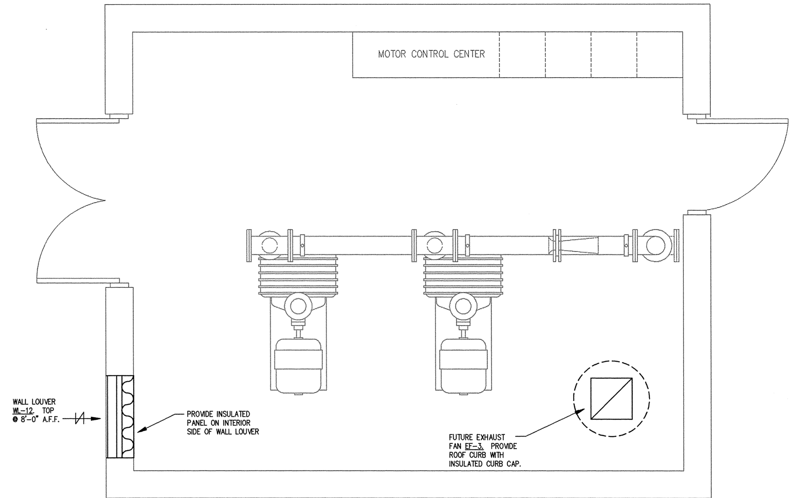
North ← 1 M3 BLOWER BUILDING MECHANICAL PLAN SCALE: 1/2"=1'-0" F.F.E. 905.00' Graphic Scale
