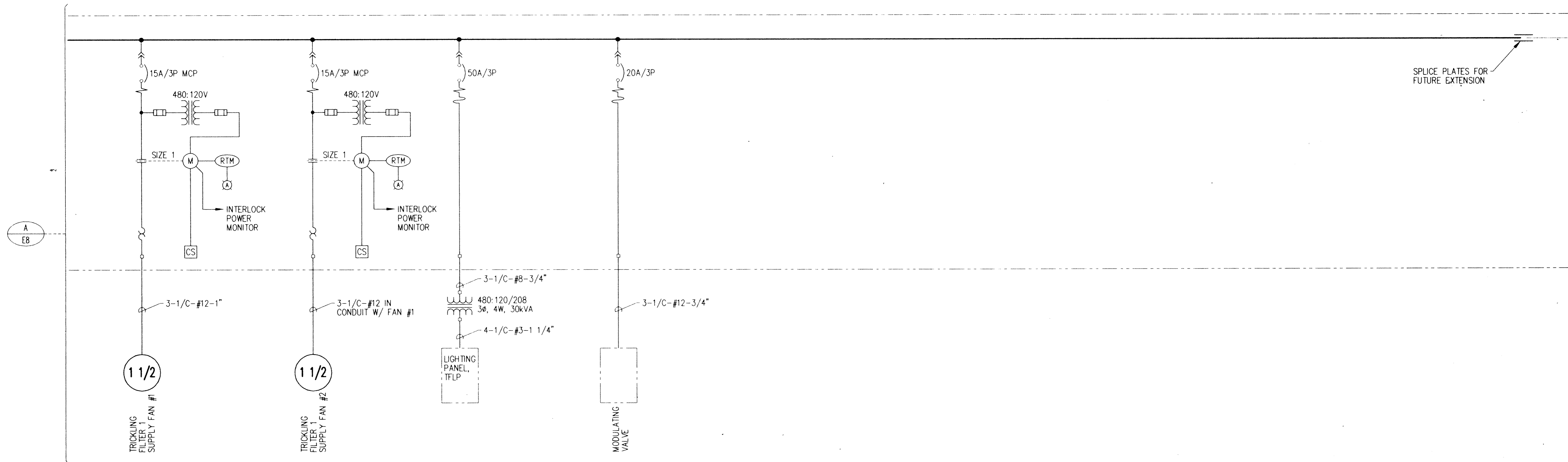
TRICKLING FILTER PUMP STATION MOTOR CONTROL CENTER (MCC) ONE-LINE DIAGRAM NO SCALE CONTINUED ABOVE & ON SHEET E9
