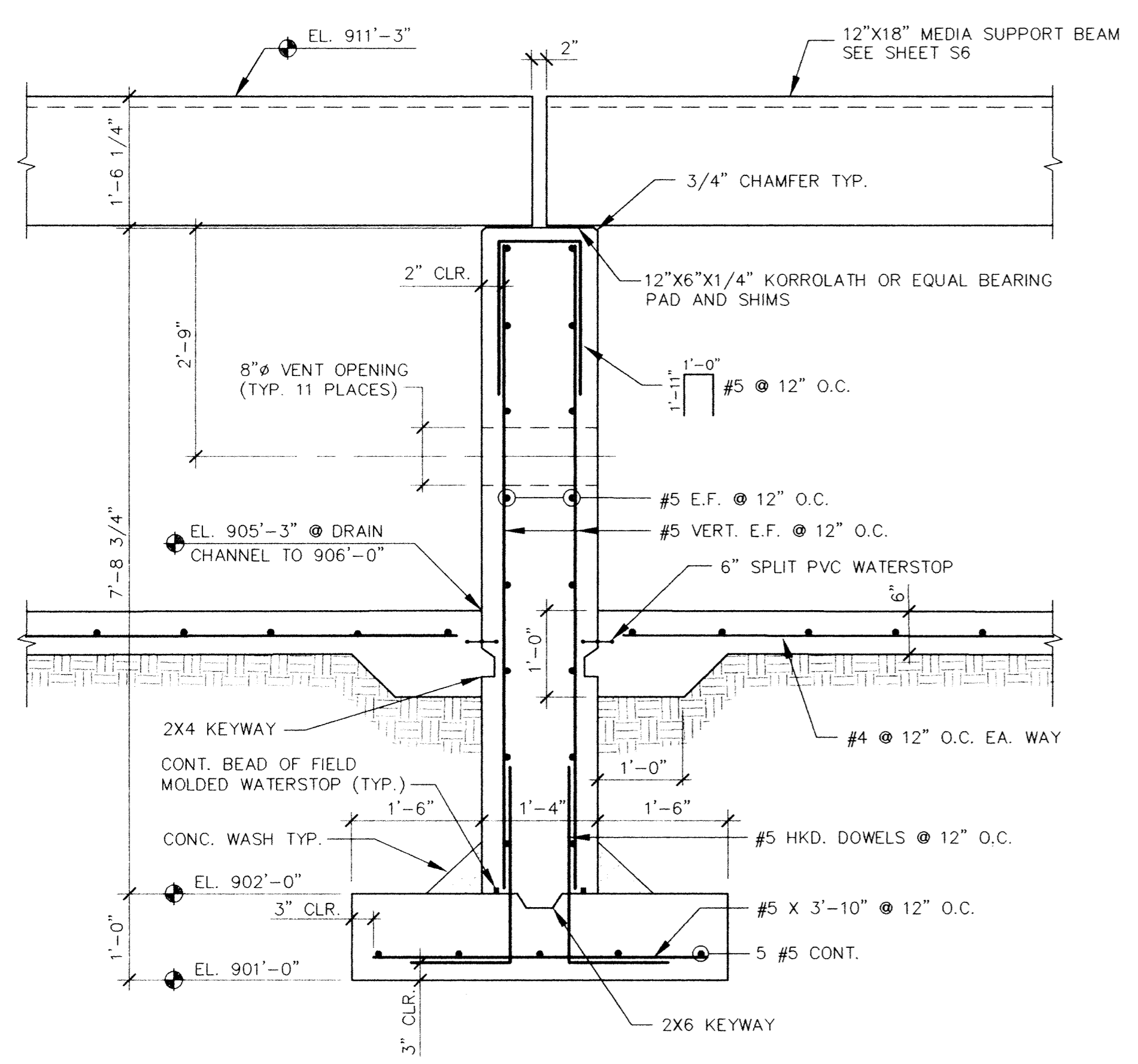
TYPICAL INTERIOR FOUNDATION WALL SECTION 6 Scale: 3/4" = 1'-0" S9
