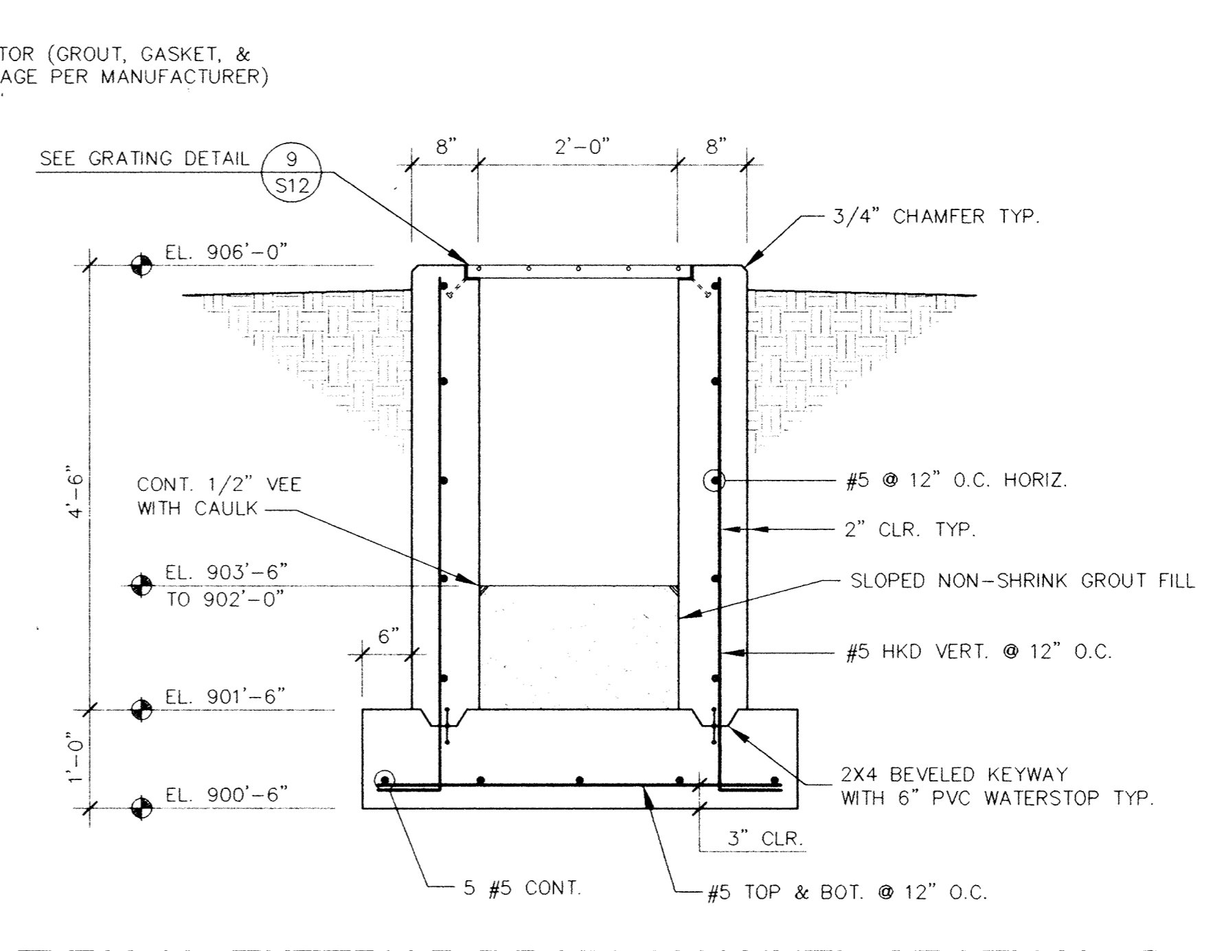
TYPICAL EXTERIOR DRAIN CHANNEL SECTION 11 Scale: 3/4" = 1'-0" S9
