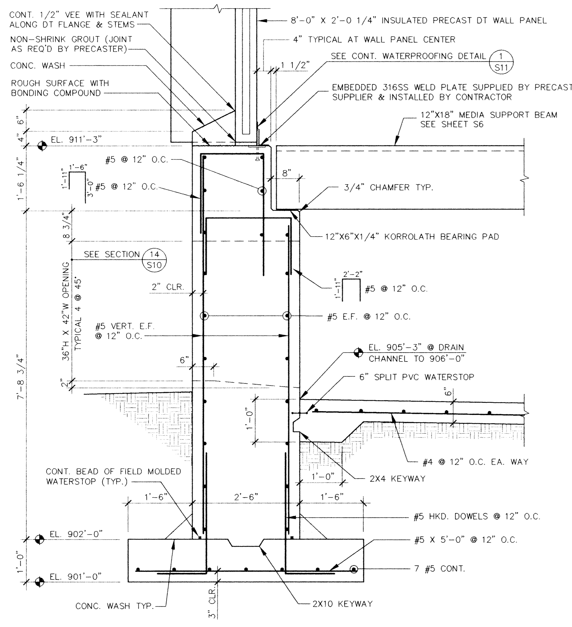
TYPICAL EXTERIOR FOUNDATION WALL SECTION 5 Scale: 3/4" = 1'-0" S9
