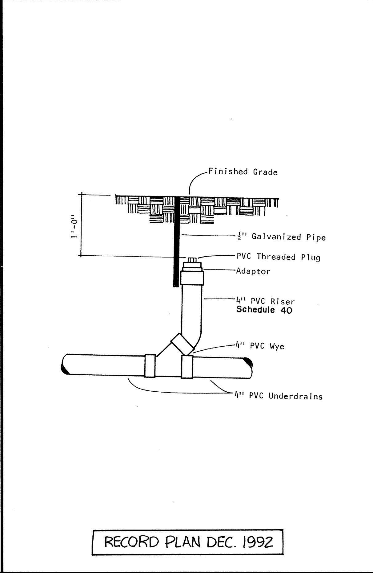
CLEANOUT
