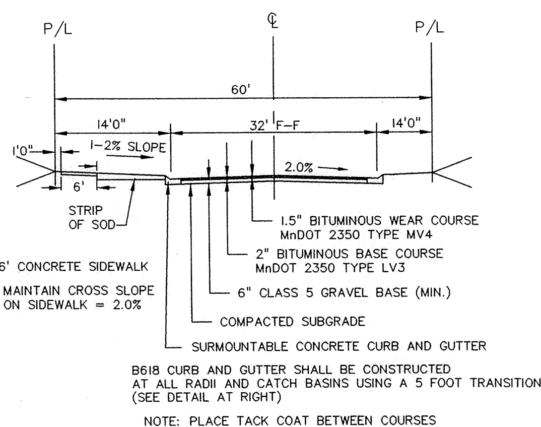
TYPICAL STREET SECTION - PUBLIC STREET
