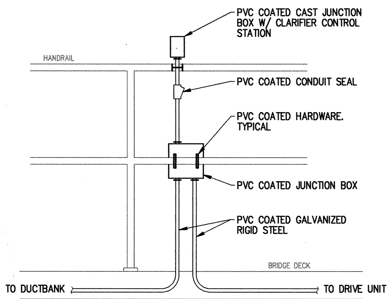
CLARIFIER CONTROL STATION DETAIL NO SCALE
