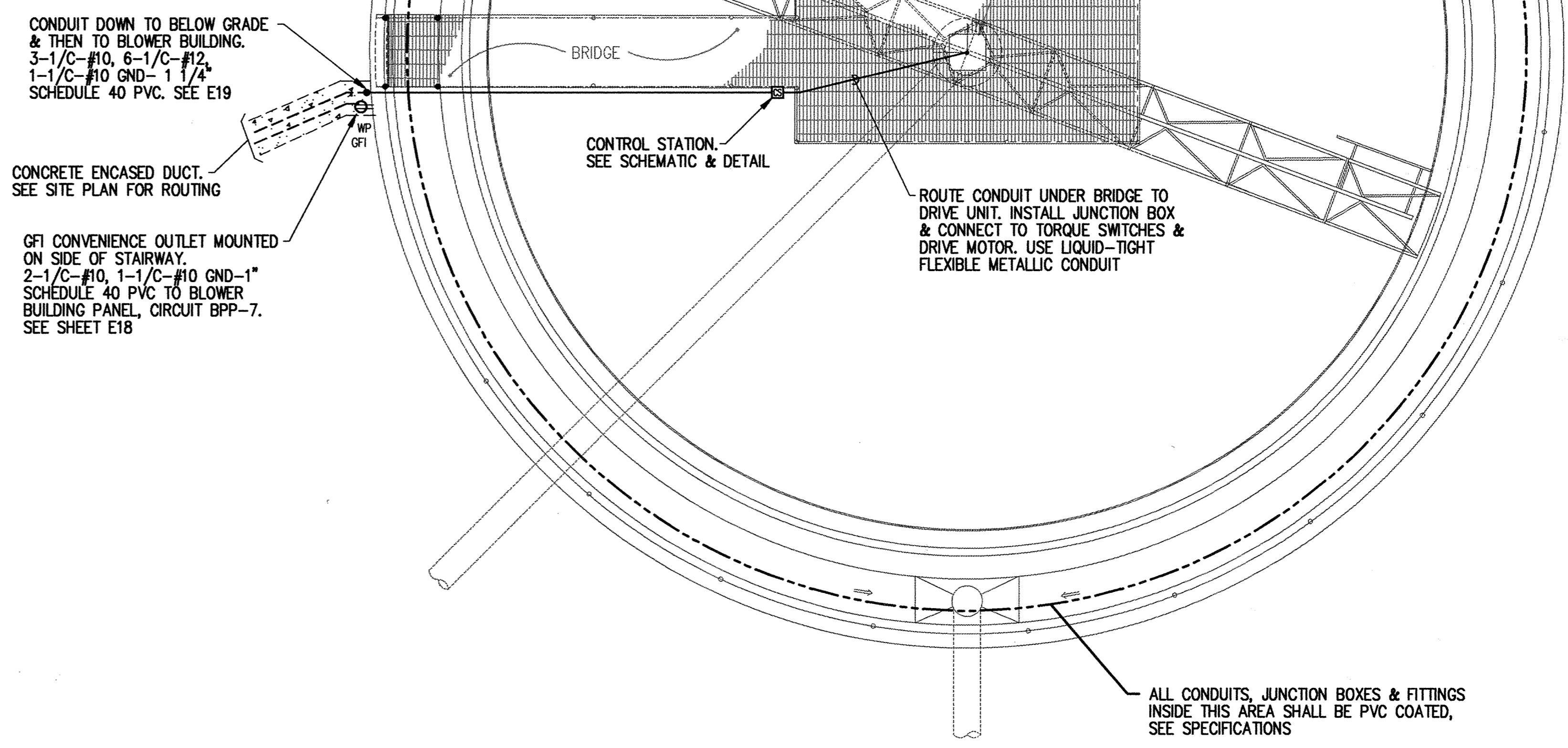
FINAL CLARIFIER ELECTRICAL PLAN SCALE: 1/4"=1'-0" TYPICAL
