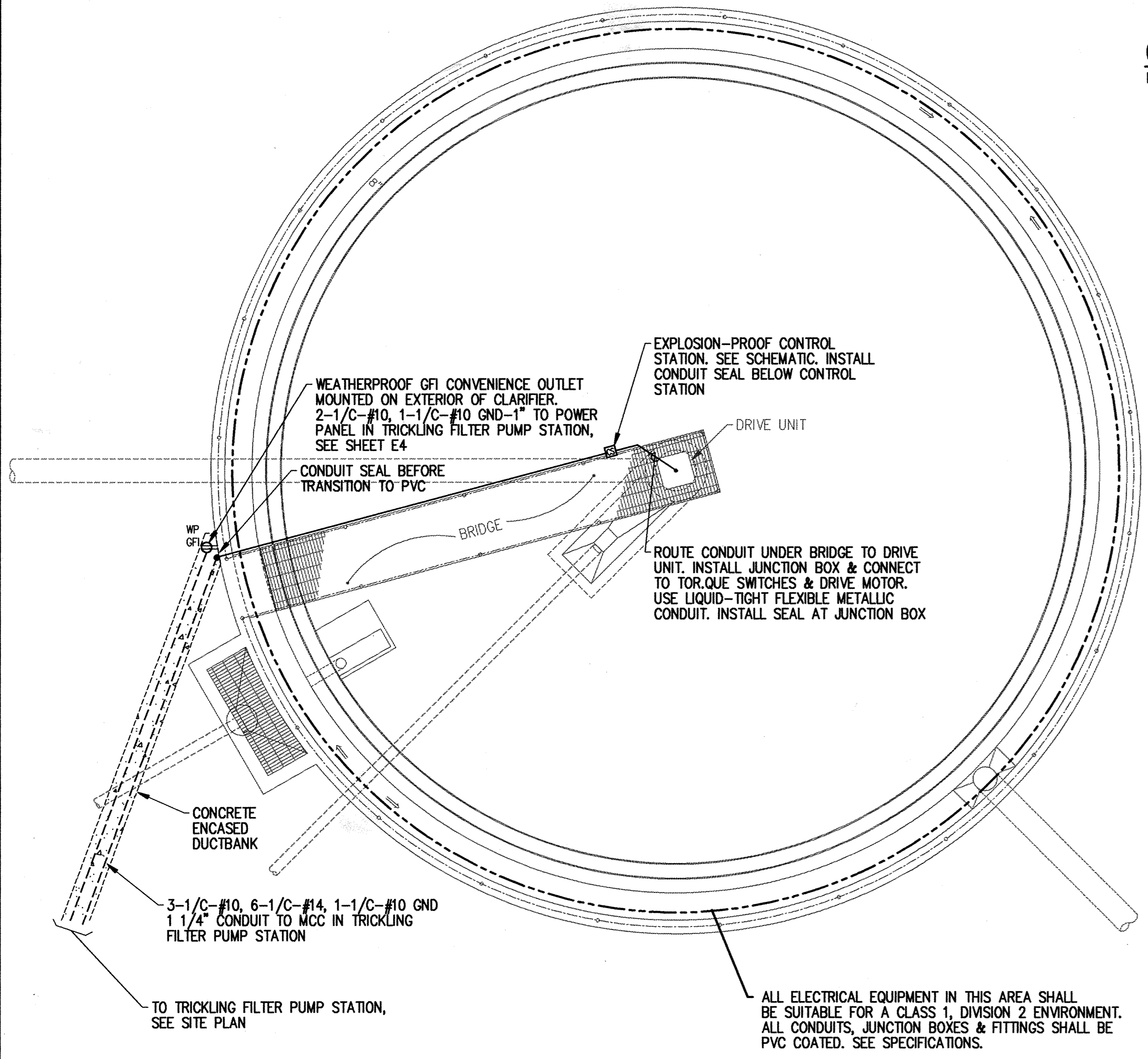
PRIMARY CLARIFIER ELECTRICAL PLAN SCALE: 1/4"=1'-0"
