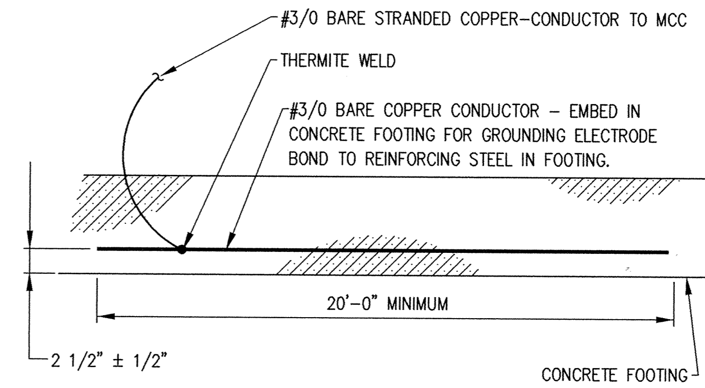
UFER GROUNDING ELECTRODE DETAIL NO SCALE
