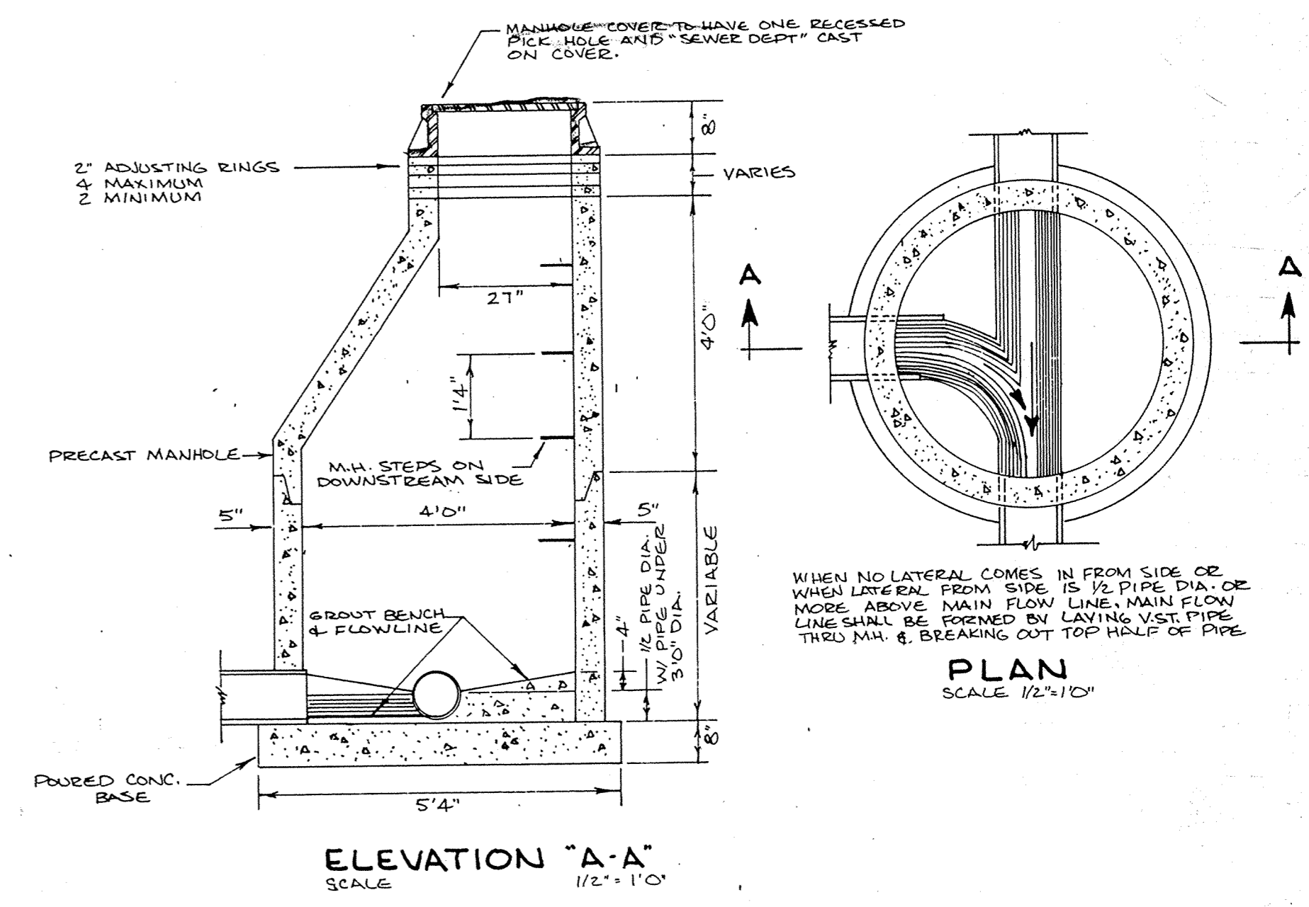
STANDARD MANHOLE DETAIL
