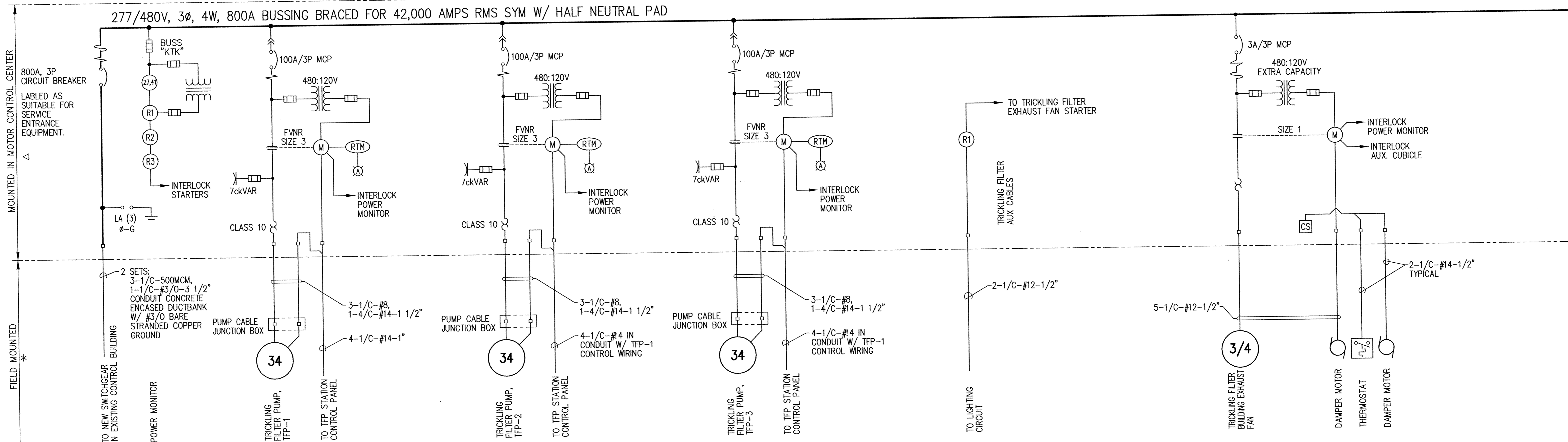
TRICKLING FILTER PUMP STATION MOTOR CONTROL CENTER (MCC) ONE-LINE DIAGRAM NO SCALE
