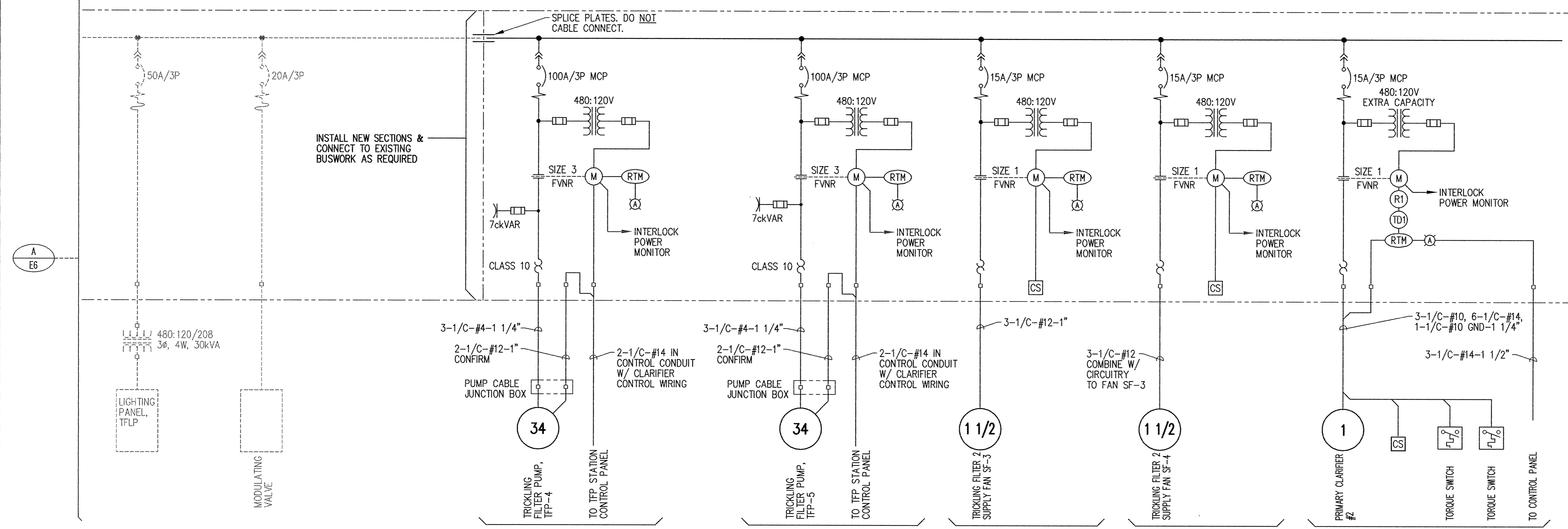
EXISTING TRICKLING FILTER PUMP STATION MOTOR CONTROL CENTER (MCC) ONE-LINE DIAGRAM MODIFICATIONS NO SCALE
