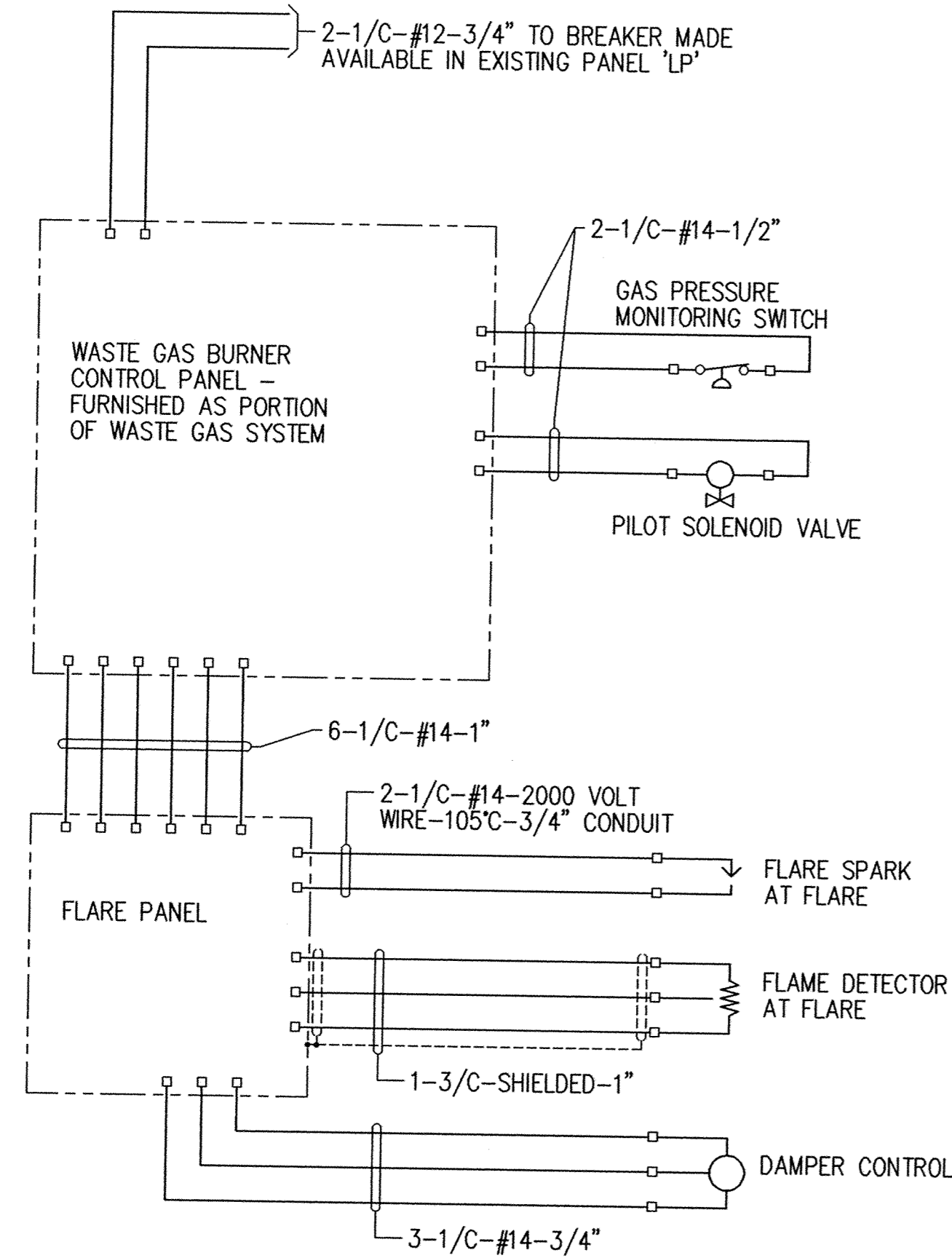
FLARE WIRING ONE-LINE DIAGRAM NO SCALE
