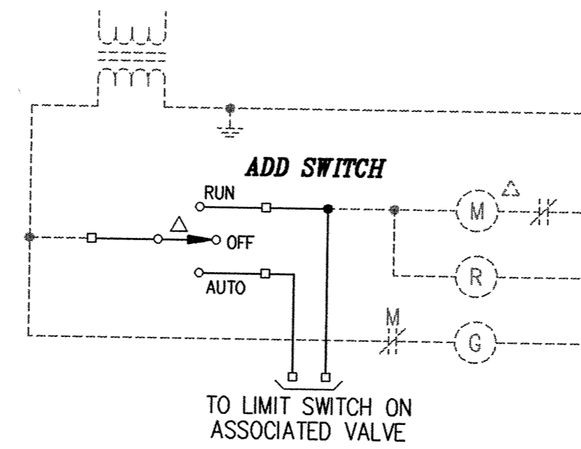
PARTIAL SCHEMATIC-REVISED DIGESTER STARTER SCHEMATIC NO SCALE SLUDGE PUMPS-TYPICAL
