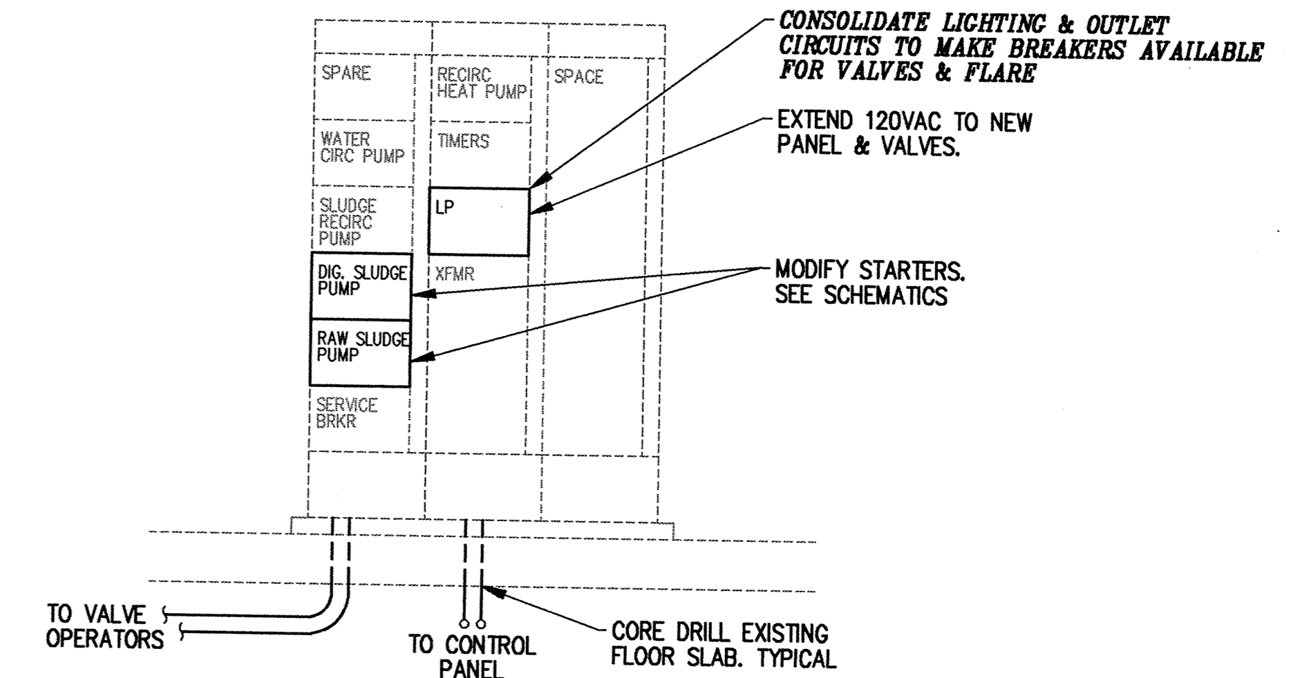
EXISTING MOTOR CONTROL CENTER ELEVATION SCALE: 1/2"=1'-0" LOCATED AT MAIN LEVEL
