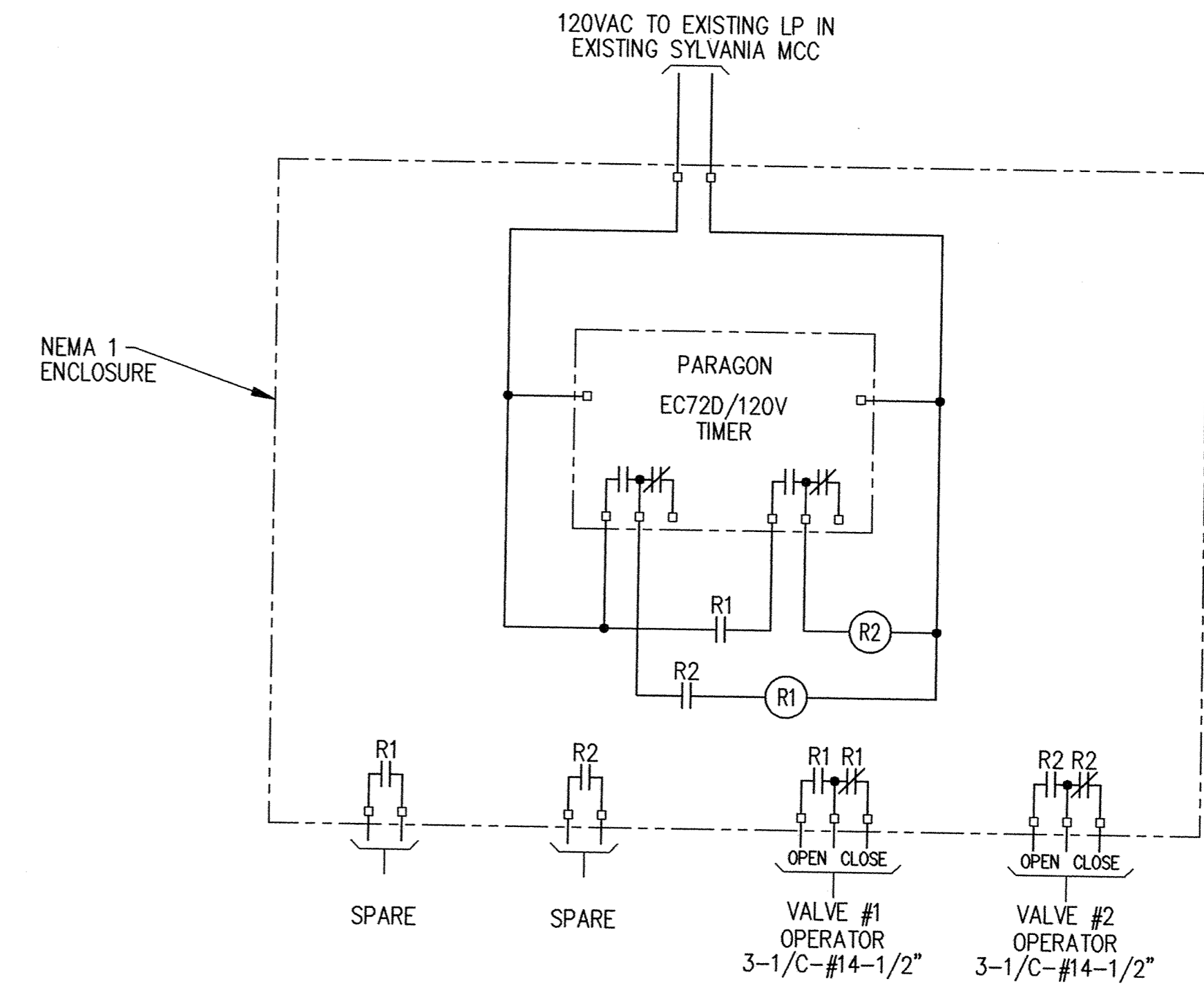
DIGESTER BUILDING CONTROL PANEL NO SCALE LOCATED AT MAIN LEVEL NEAR MCC
