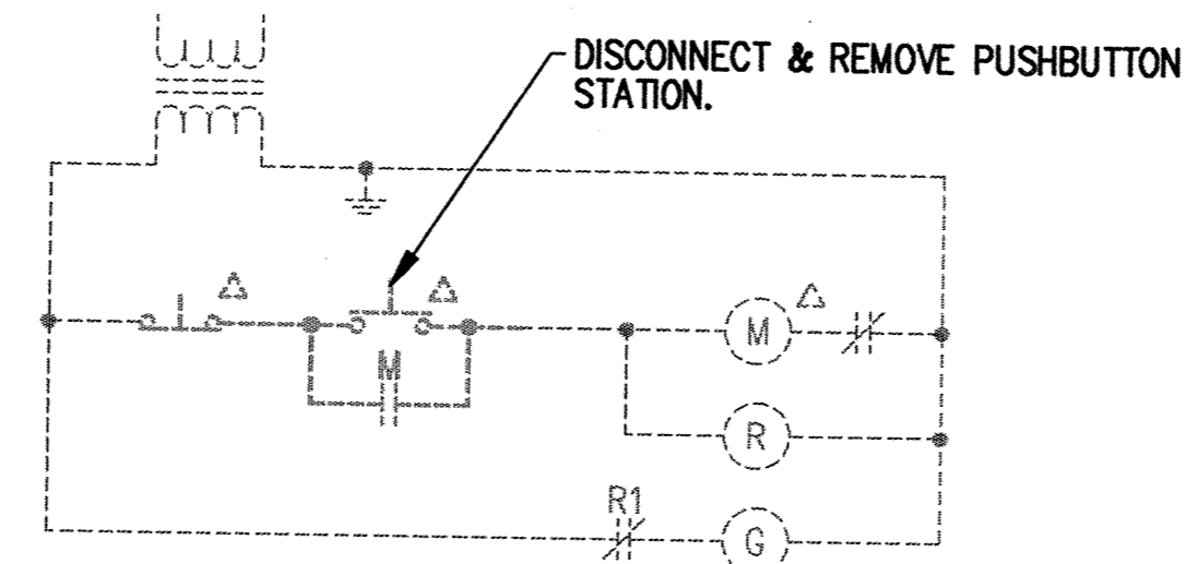
PARTIAL SCHEMATIC-EXISTING DIGESTER STARTER SCHEMATIC NO SCALE SLUDGE PUMPS-TYPICAL
