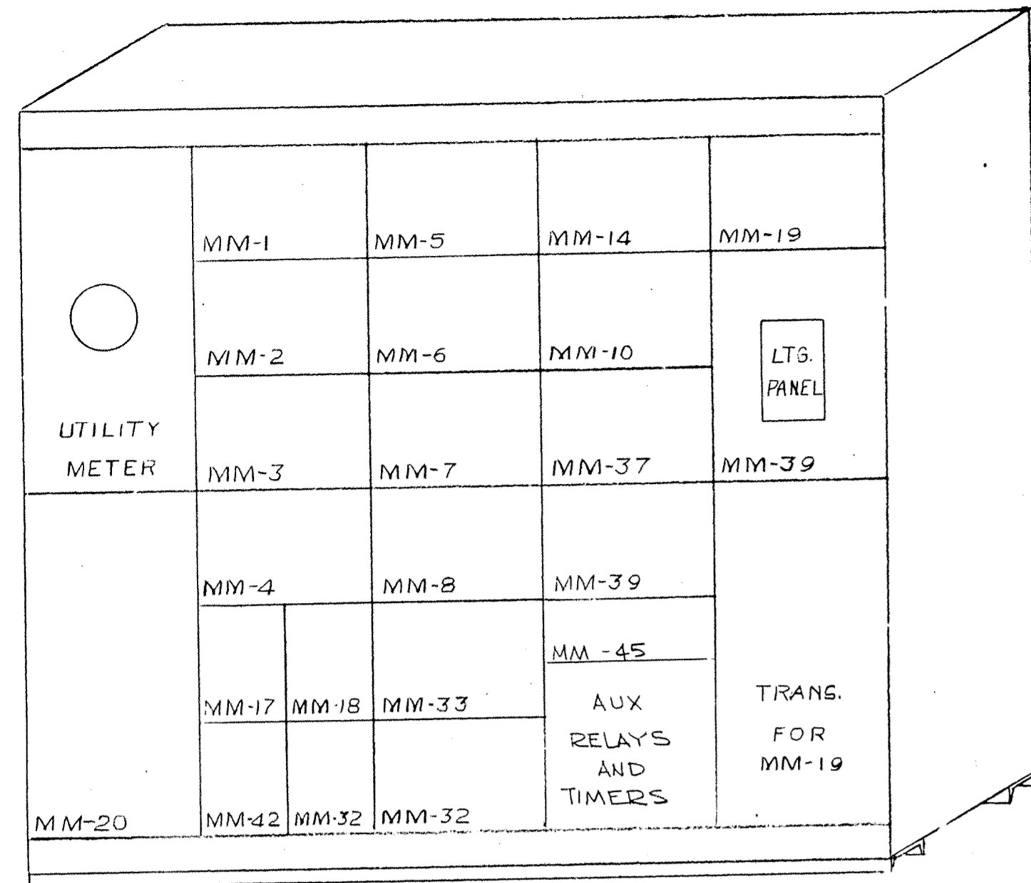
MCC-1 Not to Scale MAIN BUILDING
