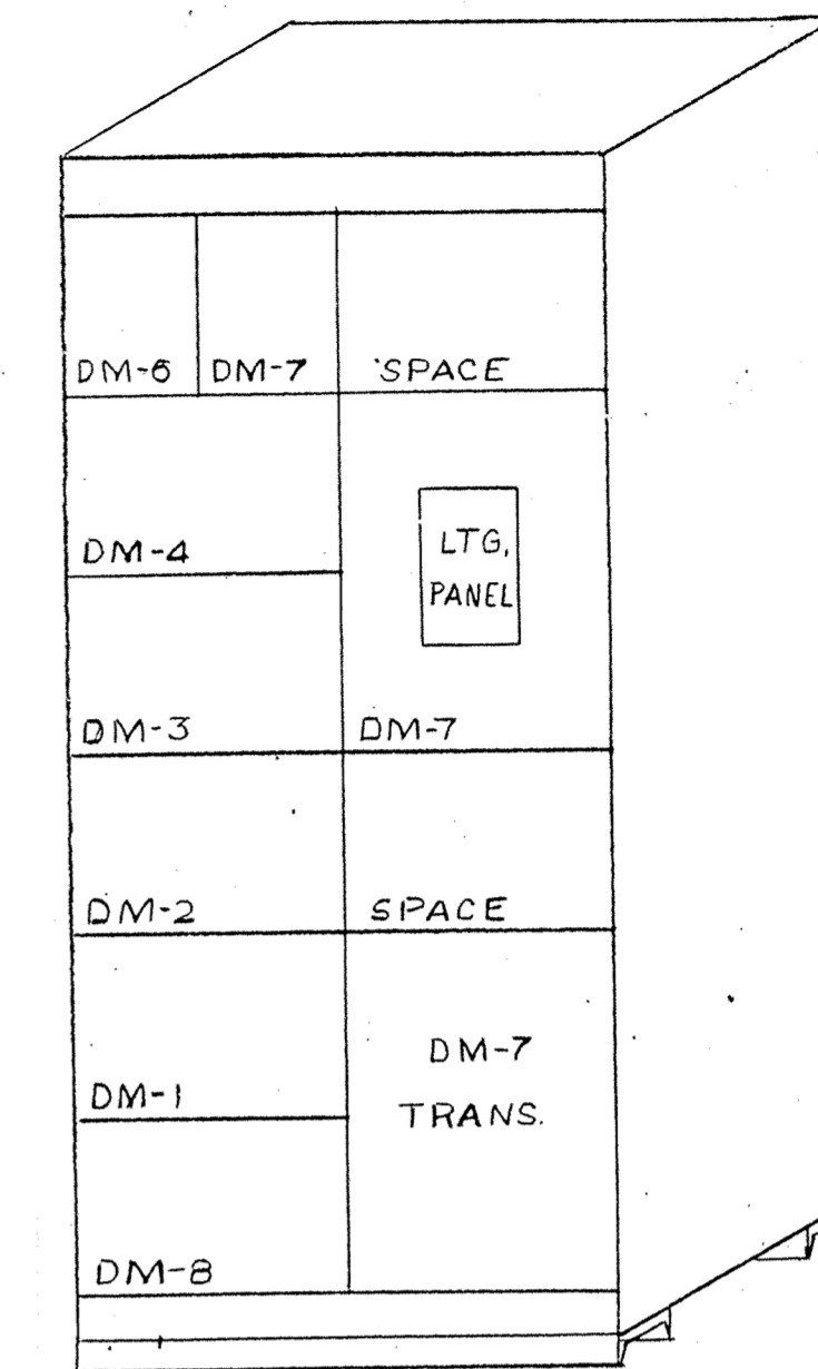
MCC-3 Not to Scale DIGESTER BUILDING
