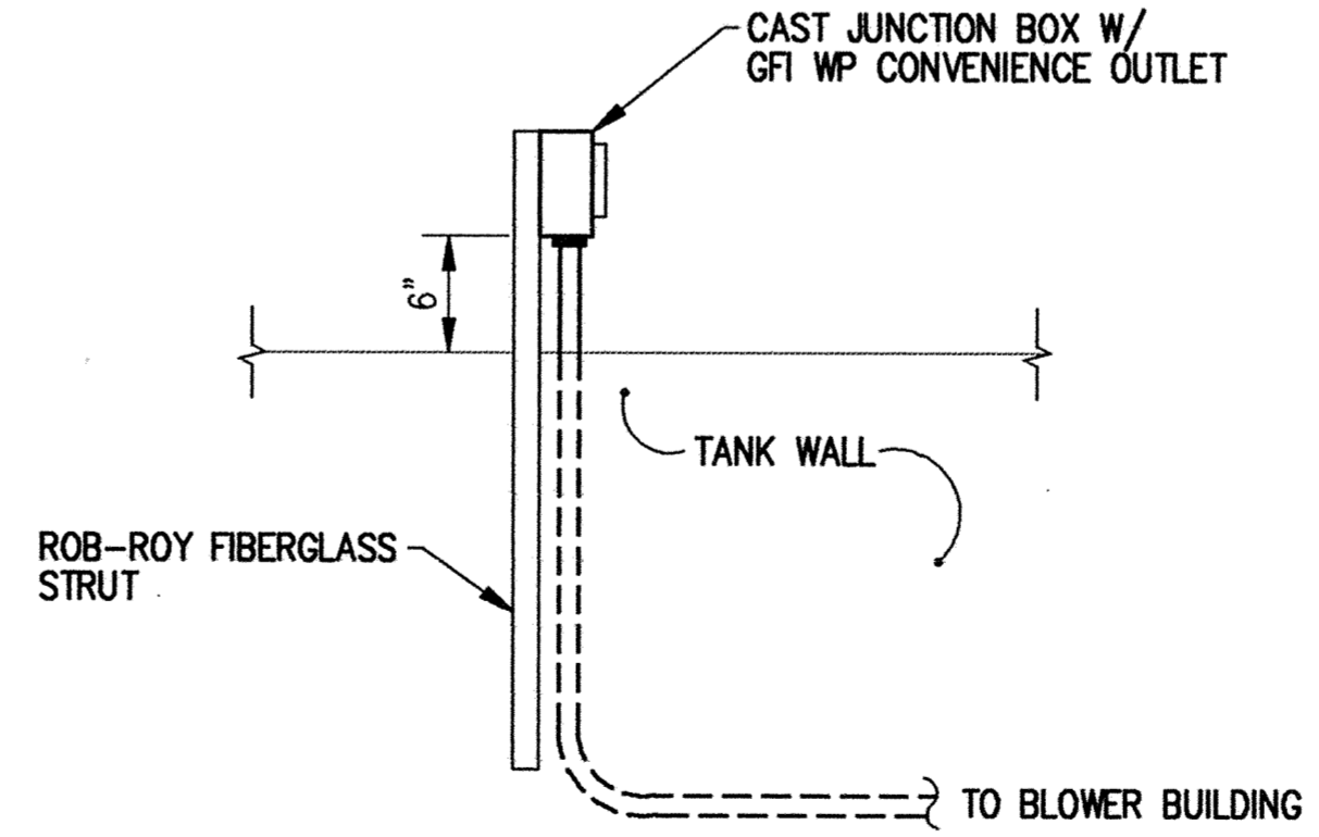
AERATION TANK OUTLET DETAIL NO SCALE
