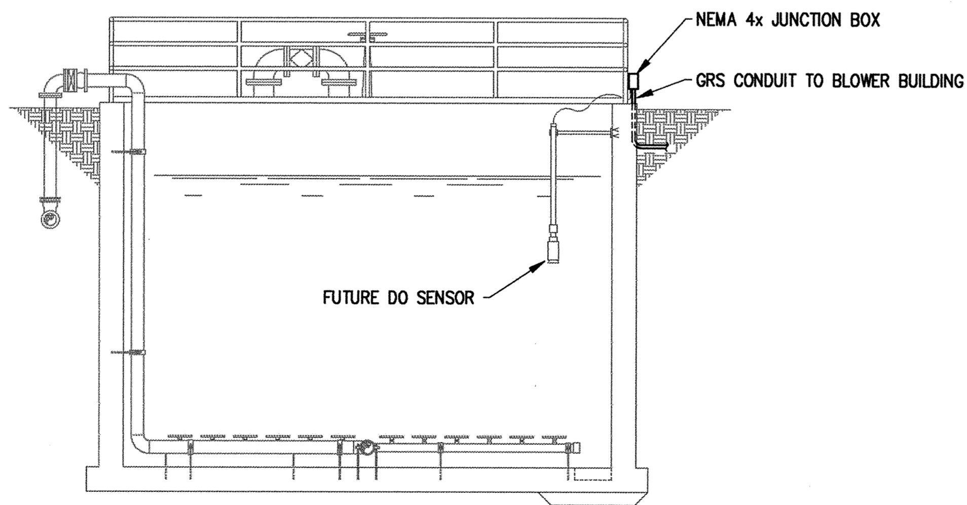
AERATION TANK ELECTRICAL SECTION SCALE: 1/4"=1'-0" 0 1 2 3 4 6 8 12 Graphic Scale
