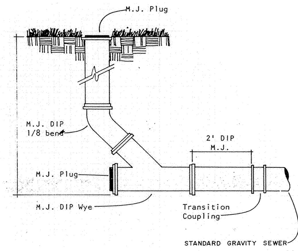
CLEANOUT DETAIL
