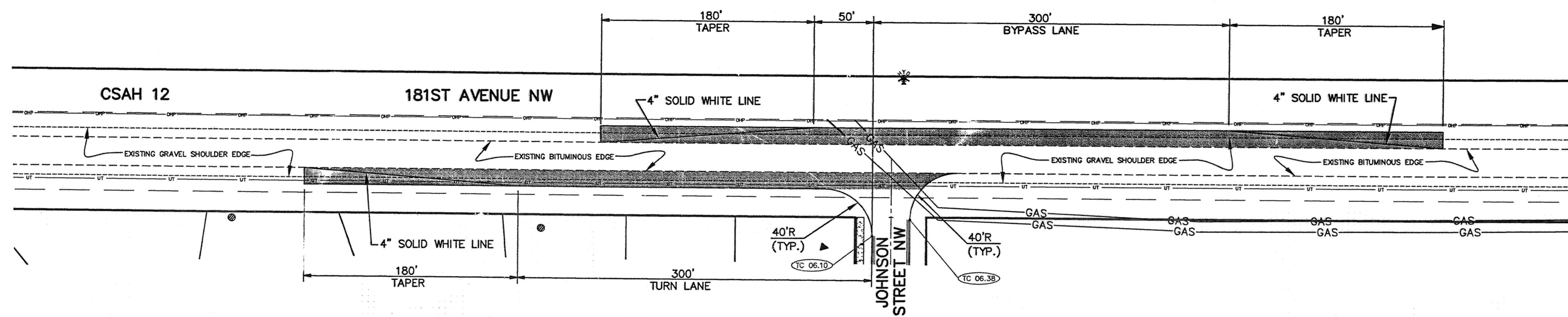
TRAFFIC CONTROL LAYOUT - 75 - 1995 MN MUTCD FIELD MANUAL
