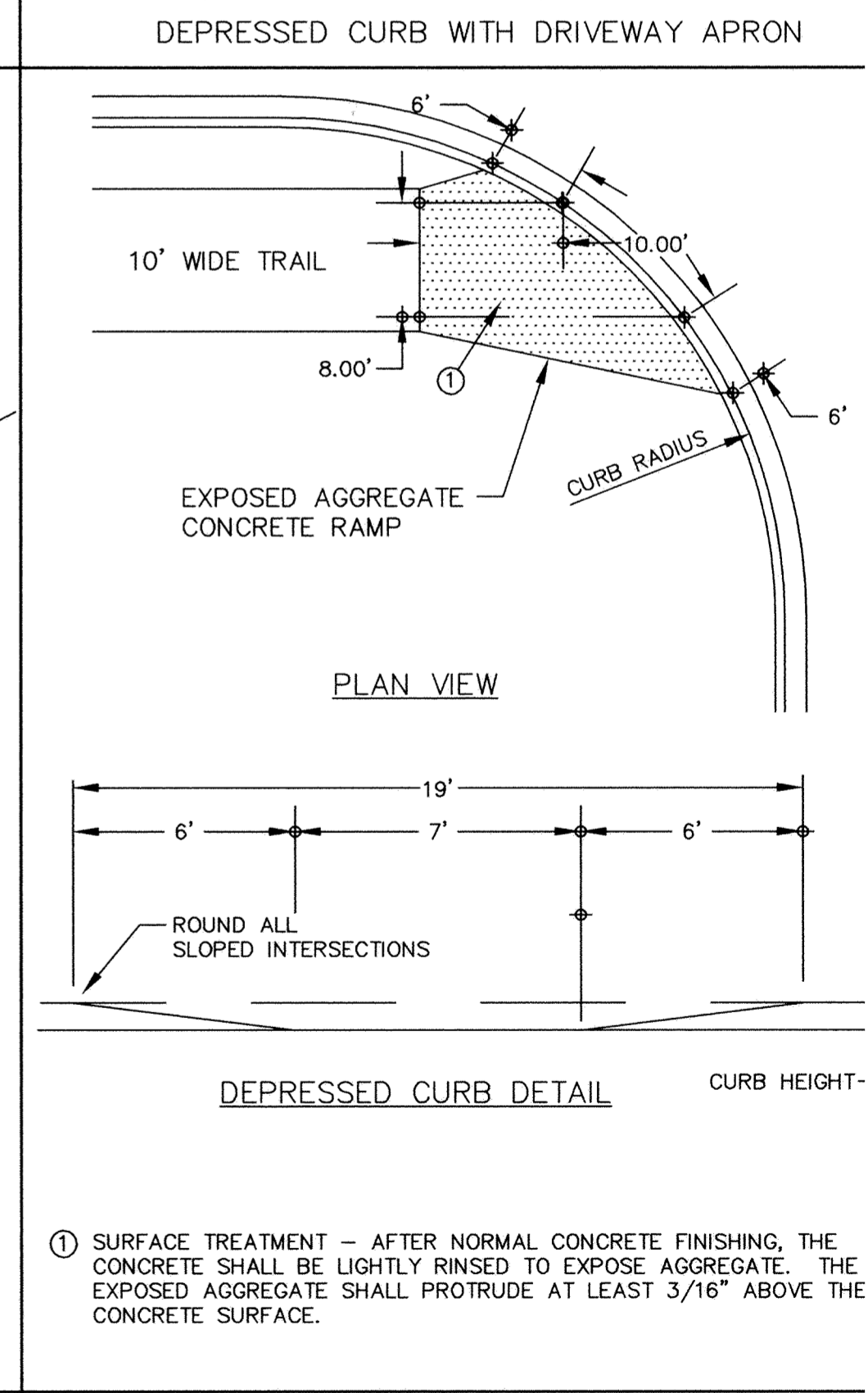
PEDESTRIAN CURB RAMPS FOR TRAILS
