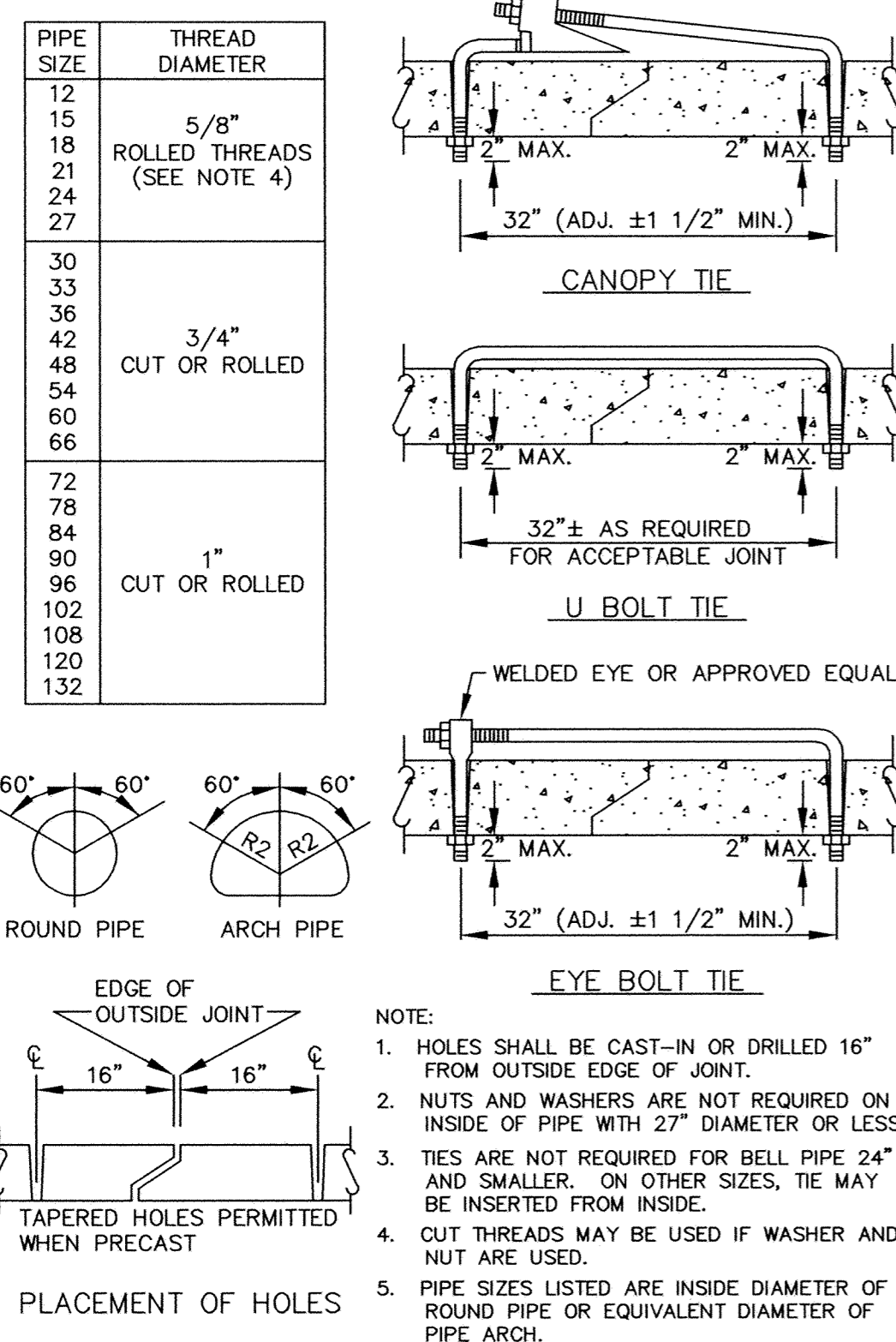
CONCRETE PIPE JOINT TIES
