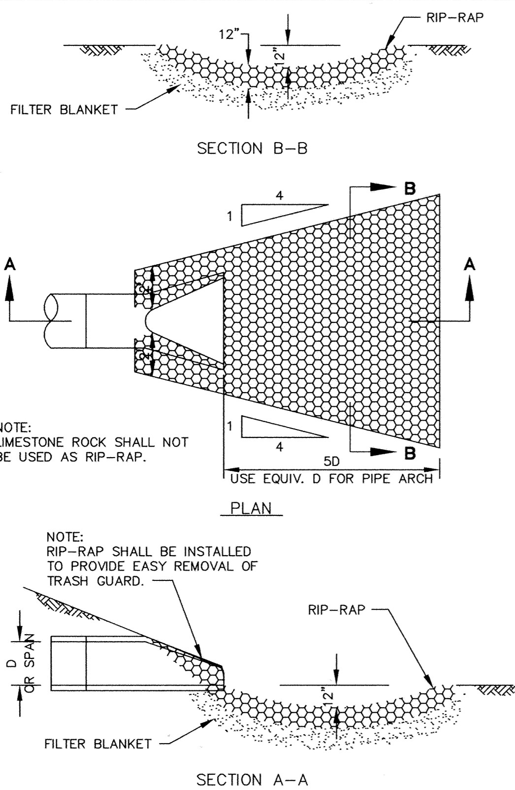
RIP-RAP INSTALLATION
