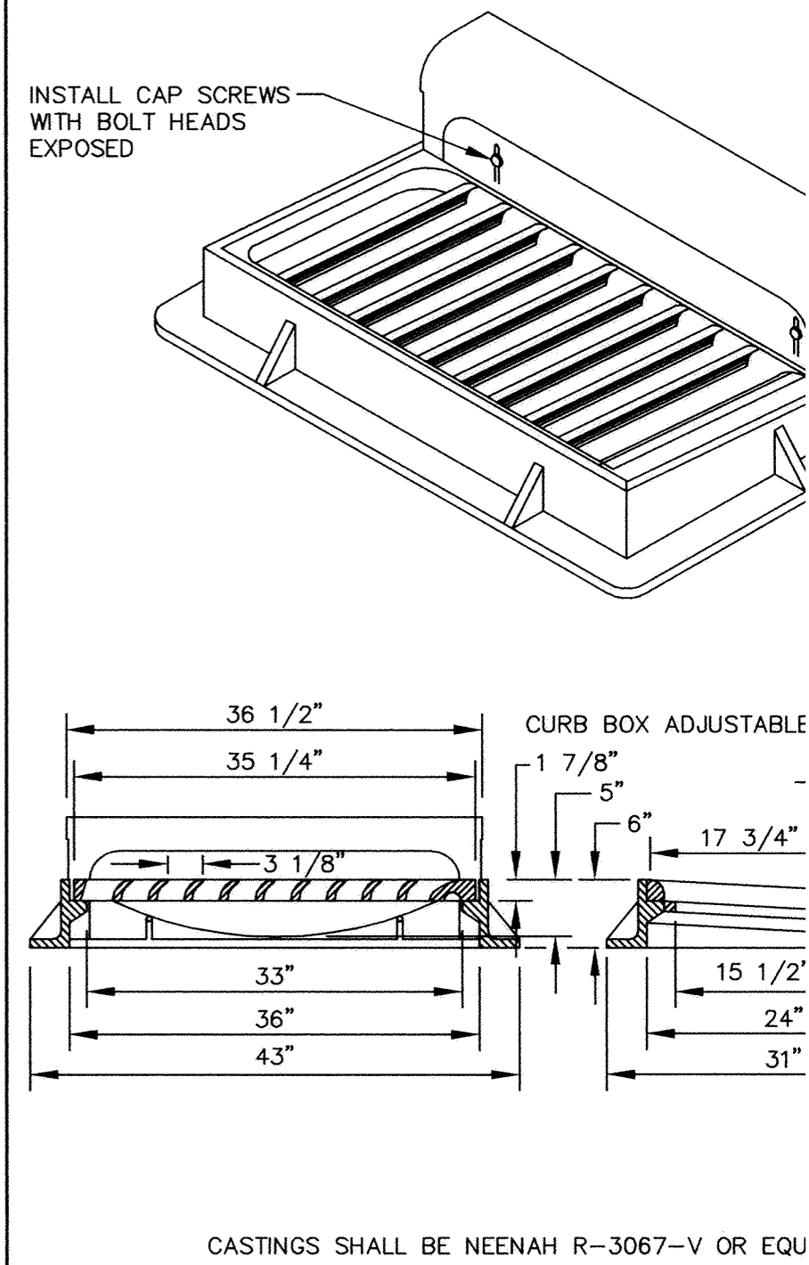
STANDARD INLET CASTING
