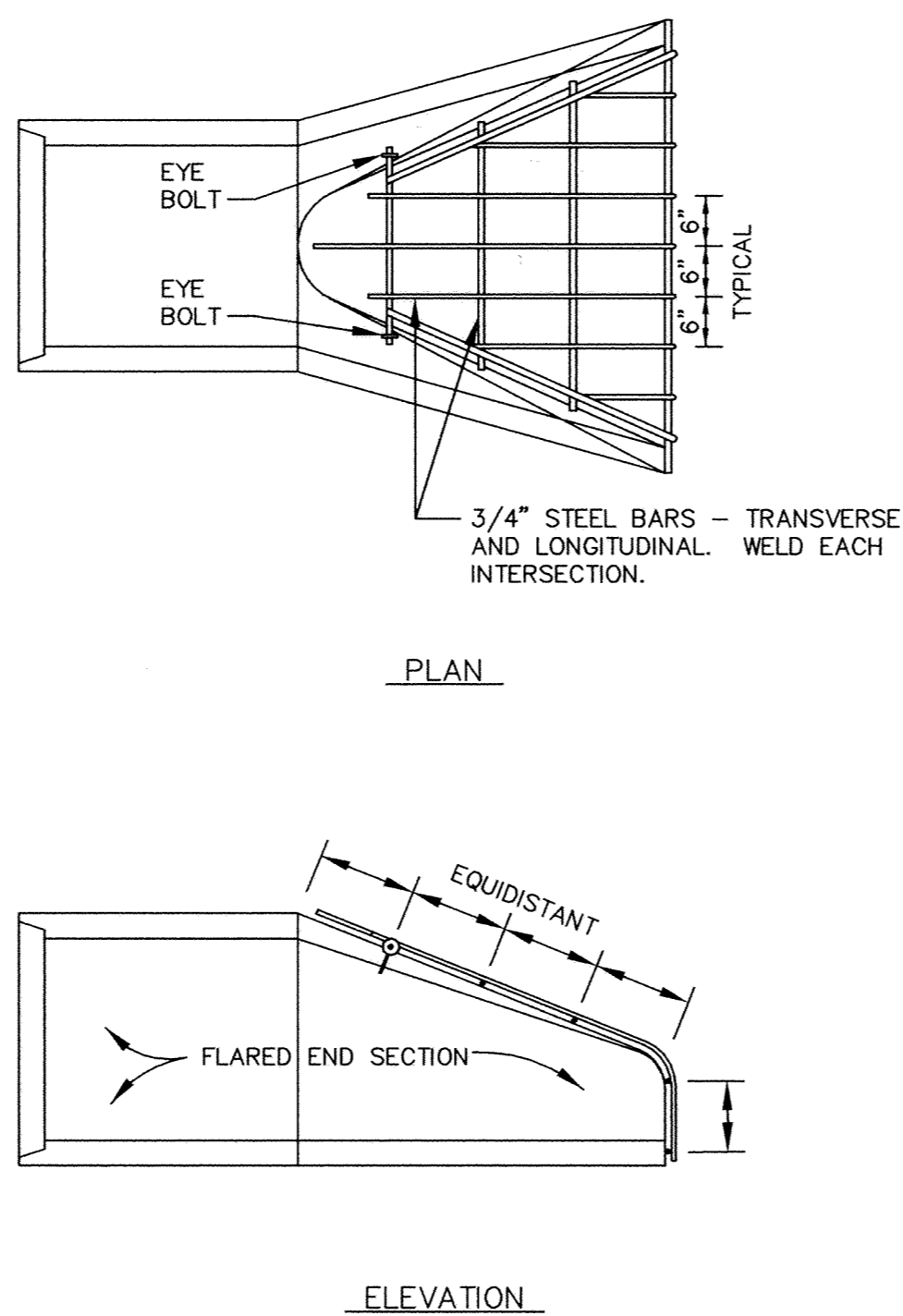
TRASH GUARD
