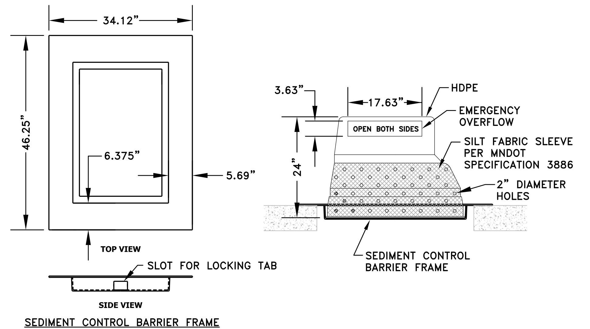
1 4 STORM DRAIN INLET PROTECTION PRE-CURB
