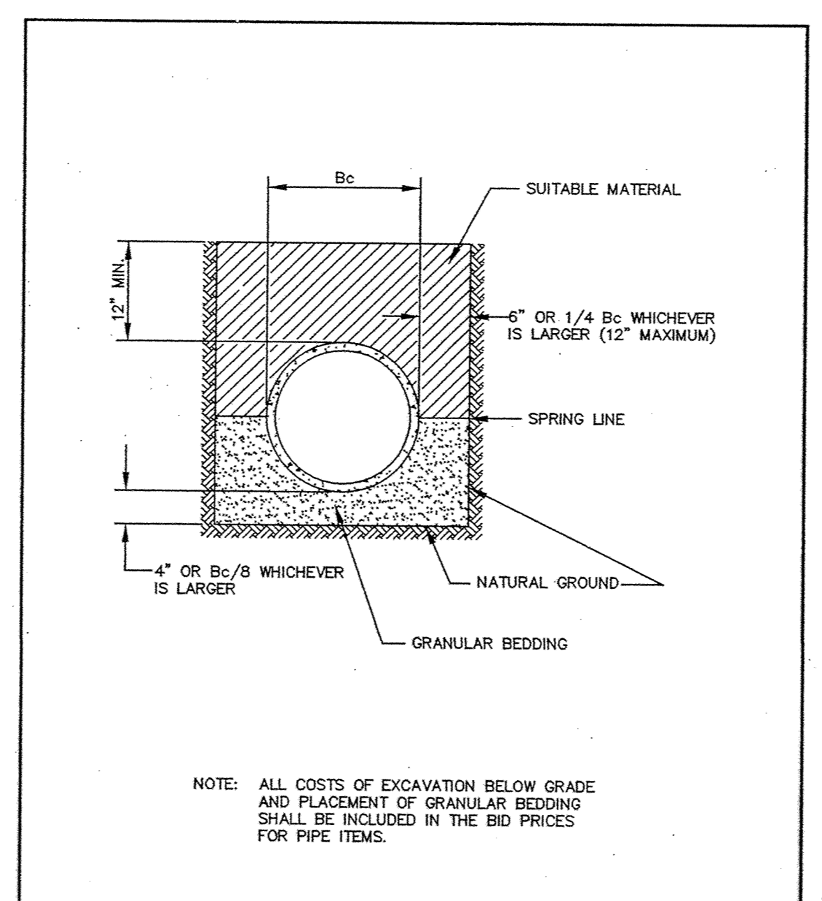
ERSTD-SA STANDARD PLATE NO. 4006 CLASS B PIPE BEDDING City of Elk River Howard R. Green Company
