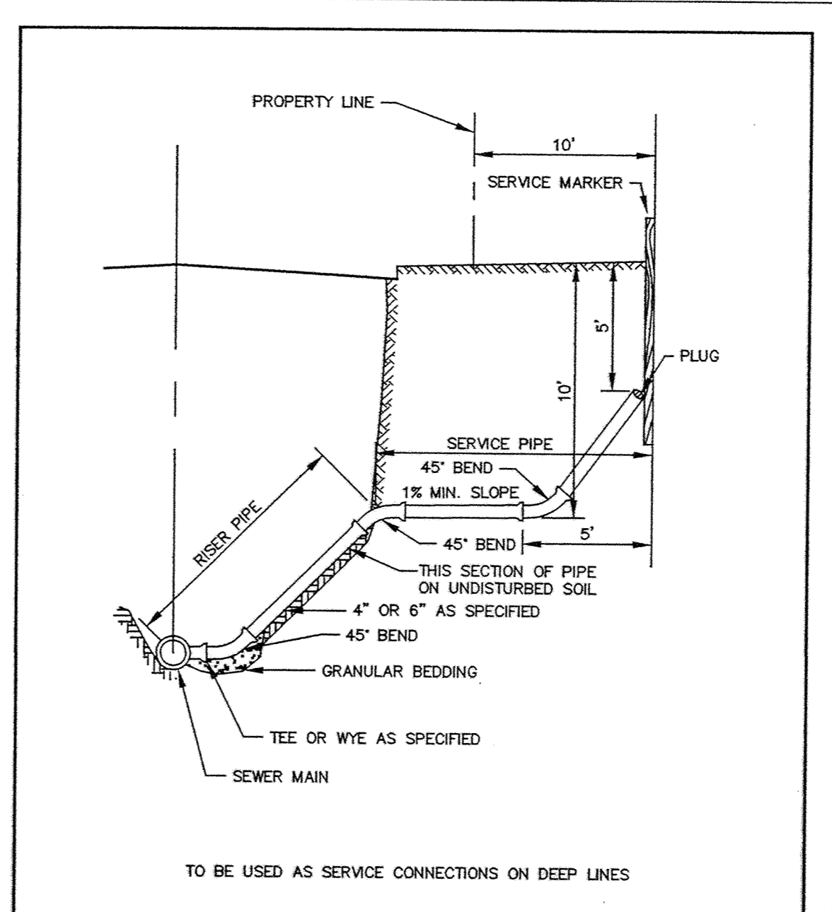
ERSTD-SA STANDARD PLATE NO. 4008 SERVICE RISER SECTION City of Elk River Howard R. Green Company
