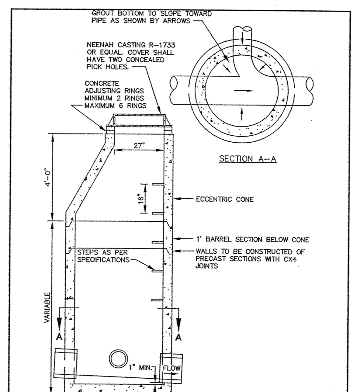
ERSTD-SA STANDARD PLATE NO. 4000 STANDARD MANHOLE City of Elk River Howard R. Green Company
