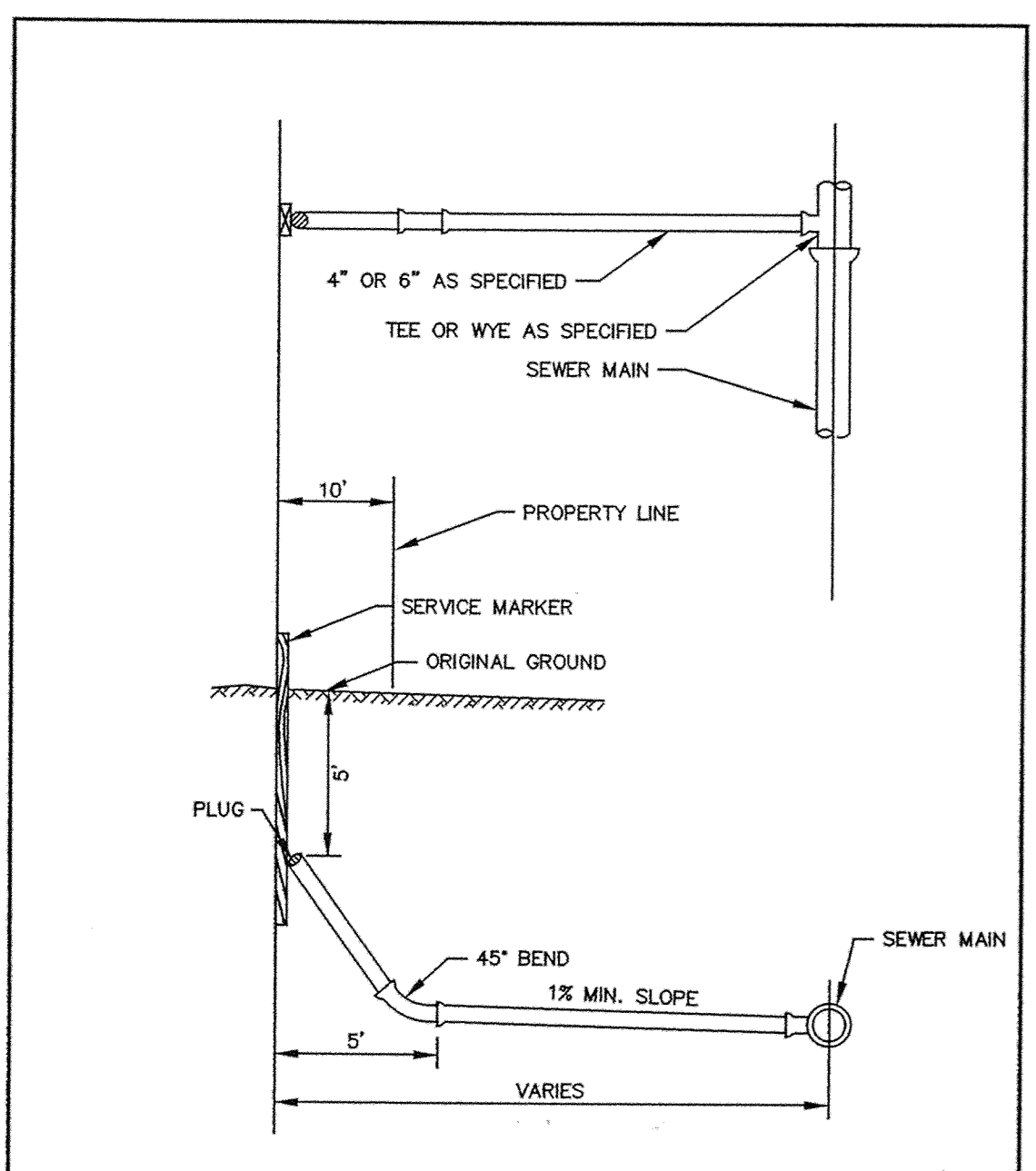
ERSTD-SA STANDARD PLATE NO. 4007 TYPICAL HOUSE SERVICE City of Elk River Howard R. Green Company
