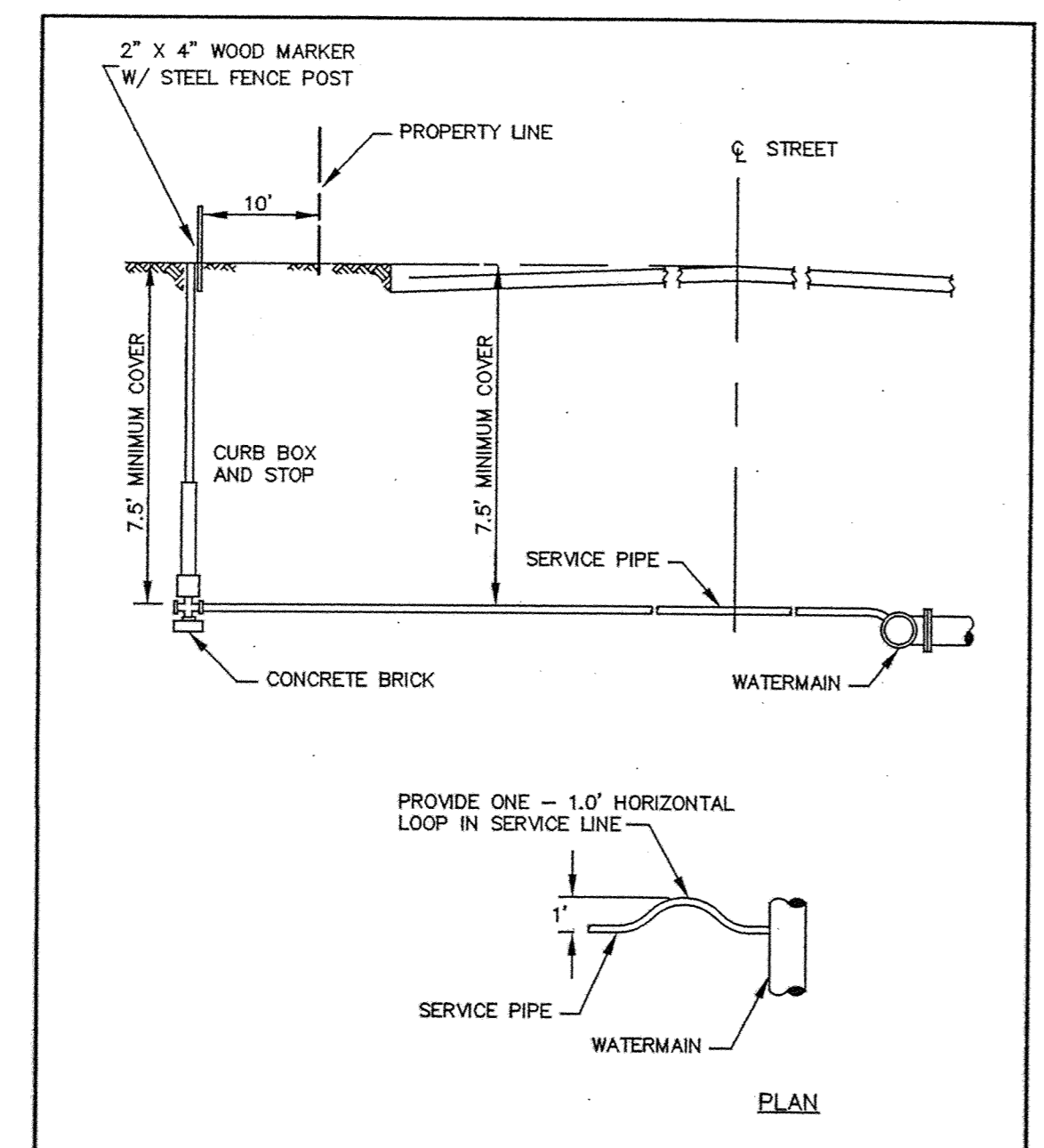
ERSTD-WM STANDARD PLATE NO. 3403 TYPICAL SERVICE DETAIL City of Elk River Howard R. Green Company
