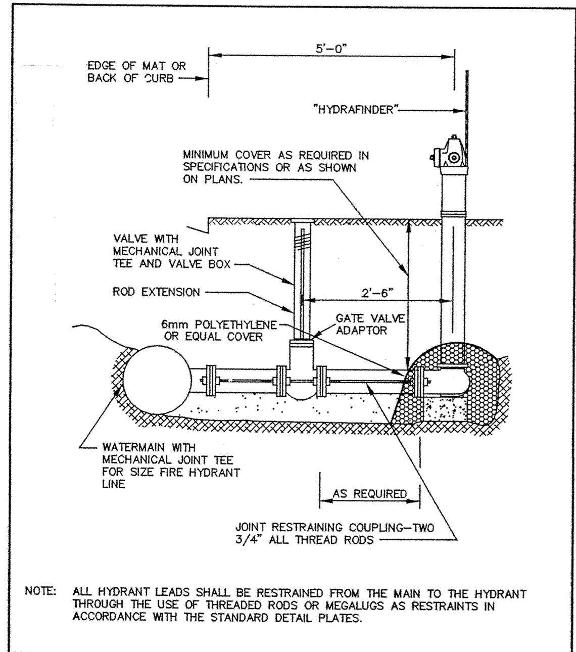
ERSTD-WM STANDARD PLATE NO. 3402 RODDING DETAIL City of Elk River Howard R. Green Company
