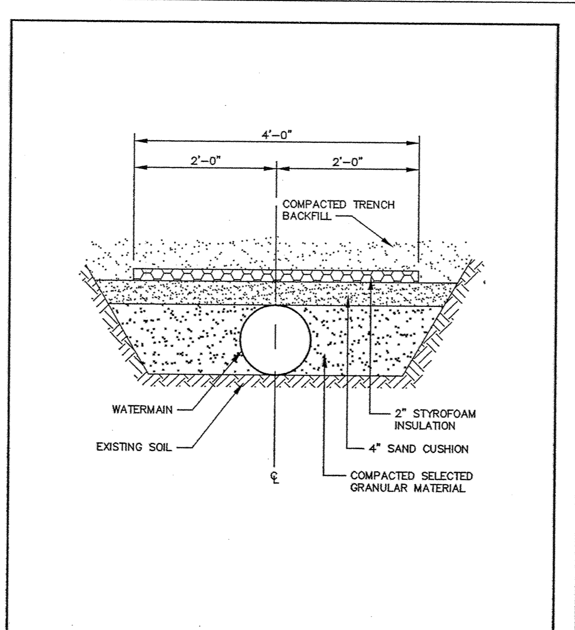
ERSTD-WM STANDARD PLATE NO. 3407 PIPE INSULATION DETAIL City of Elk River Howard R. Green Company
