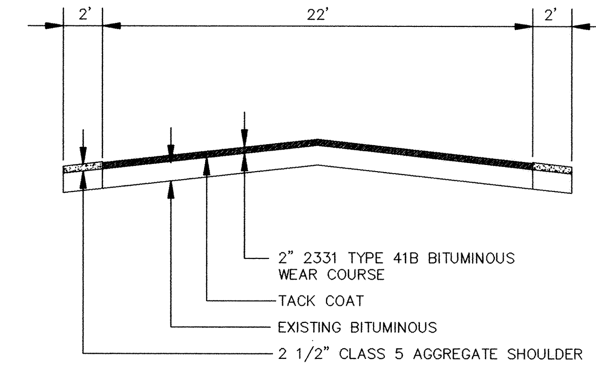
TYPICAL STREET SECTION 165TH AVENUE
